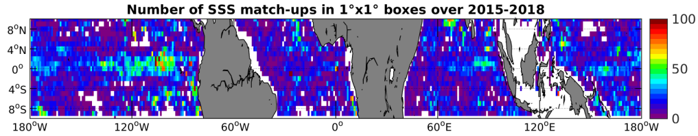
Figure 4: Number of SSS match-ups between Argo SSS and the SMAP-L3-RSS-V2-MONTHLY-70KM SSS product for the Equatorial Ocean 10N-10S Pi-MEP region over 1^\circ \times 1^\circ boxes and for the full satellite product period.
