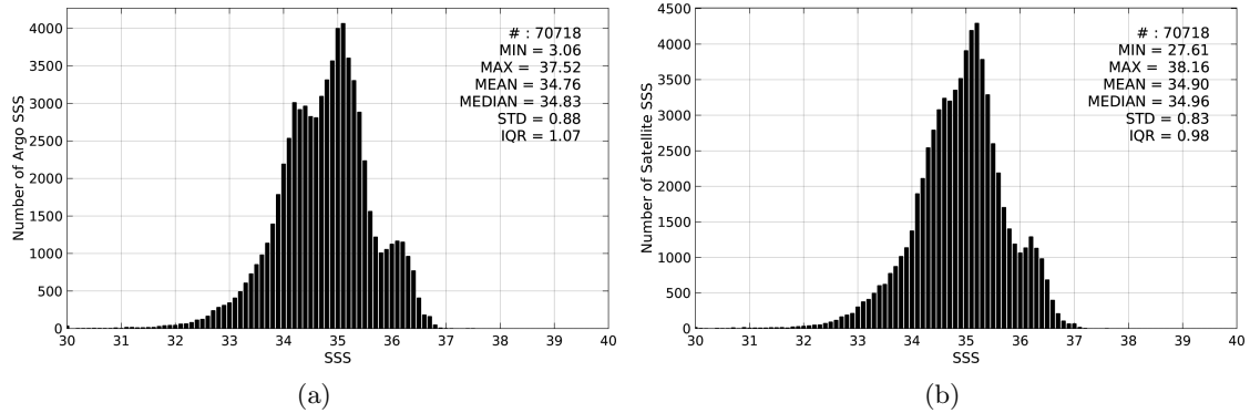
Figure 2: Histograms of SSS from Argo (a) and SMAP-L3-RSS-V2-MONTHLY-70KM (b) considering all match-up pairs per bins of 0.1 over the Equatorial Ocean 10N-10S Pi-MEP region and for the full satellite product period.
