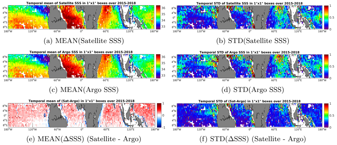
Figure 6: Temporal mean (left) and STD (right) of SSS from SMAP-L3-RSS-V2-MONTHLY-70KM (top), Argo (middle), and of \Delta SSS (Satellite - Argo). Only match-up pairs are used to generate these maps.
