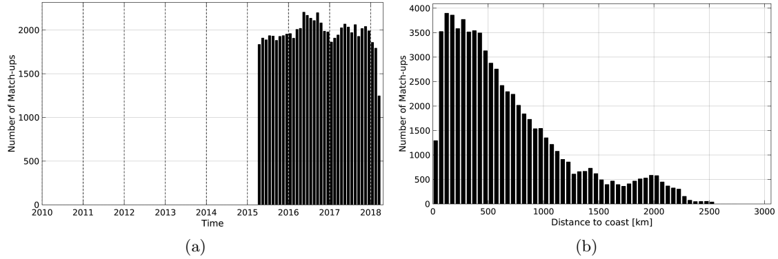
Figure 1: Number of match-ups between Argo and SMAP-L3-RSS-V2-MONTHLY-70KM SSS as a function of time (a) and as function of the distance to coast (b) over the Equatorial Ocean 10N-10S Pi-MEP region and for the full satellite product period.
