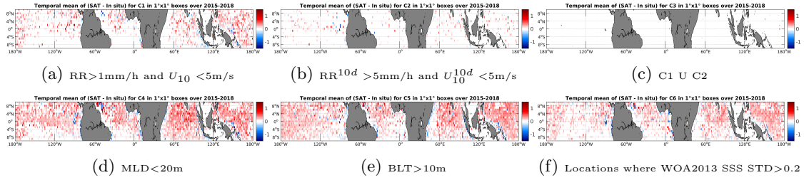
Figure 12: Temporal mean gridded over spatial boxes of size 1^\circ \times 1^\circ of \Delta SSS (SMAP-L3-RSS-V2-MONTHLY-70KM - Argo) for 6 different subdatasets corresponding to: RR > 1\text{mm/h} and U_{10} < 5\text{m/s} (a), RR^{10d} > 5\text{mm/h} and U_{10}^{10d} < 5\text{m/s} (b), C1 U C2 (c), MLD < 20\text{m} (d), BLT > 10\text{m} (e), Locations where WOA2013 SSS STD > 0.2 (f).
