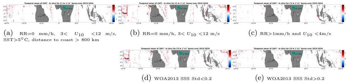
Figure 14: Temporal mean gridded over spatial boxes of size 1^\circ \times 1^\circ of \Delta\text{SSS} (SMAP SSS L3 v5.0 - 8-Day running (JPL) - TSG (SAMOS)) for 5 different subdatasets corresponding to: RR=0 mm/h, 3 < U_{10} < 12 m/s, SST>5°C, distance to coast > 800 km (a), RR=0 mm/h, 3 < U_{10} < 12 m/s (b), RR>1mm/h and U_{10} < 4 m/s (c), WOA2013 SSS Std<0.2 (d), WOA2013 SSS Std>0.2 (e).
