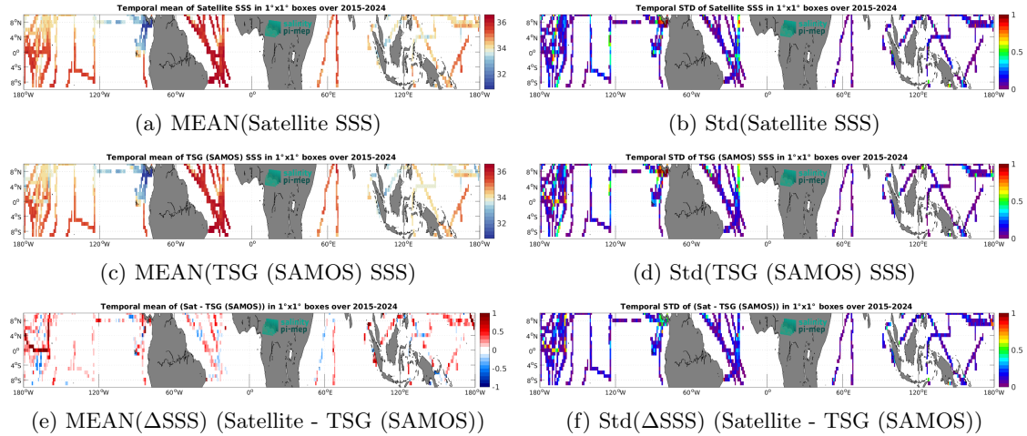
Figure 7: Temporal mean (left) and Std (right) of SSS from SMAP SSS L3 v5.0 - 8-Day running (JPL) (top), TSG (SAMOS) (middle), and of \Delta SSS (Satellite - TSG (SAMOS)). Only match-up pairs are used to generate these maps.
