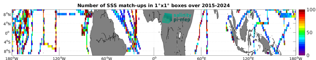
Figure 5: Number of SSS match-ups between TSG (SAMOS) SSS and the SMAP SSS L3 v5.0 - 8-Day running (JPL) SSS product for the Equatorial Ocean 10N-10S Pi-MEP region over 1^\circ \times 1^\circ boxes and for the full satellite product period.
