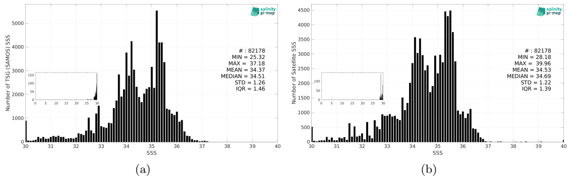
Figure 3: Histograms of SSS from TSG (SAMOS) (a) and SMAP SSS L3 v5.0 - 8-Day running (JPL) (b) considering all match-up pairs per bins of 0.1 over the Equatorial Ocean 10N-10S Pi-MEP region and for the full satellite product period.
