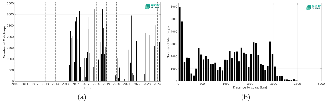
Figure 2: Number of match-ups between TSG (SAMOS) and SMAP SSS L3 v5.0 - 8-Day running (JPL) SSS as a function of time (a) and as function of the distance to coast (b) over the Equatorial Ocean 10N-10S Pi-MEP region and for the full satellite product period.
