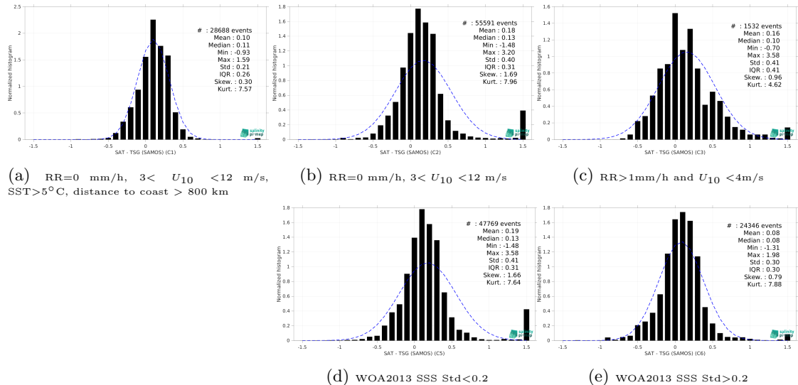
Figure 15: Normalized histogram of \Delta SSS (SMAP SSS L3 v5.0 - 8-Day running (JPL) - TSG (SAMOS)) for 5 different subdatasets corresponding to: RR=0 mm/h, 3 < U_{10} < 12 m/s, SST>5°C, distance to coast > 800 km (a), RR=0 mm/h, 3 < U_{10} < 12 m/s (b), RR>1mm/h and U_{10} < 4 m/s (c), WOA2013 SSS Std<0.2 (d), WOA2013 SSS Std>0.2 (e).
