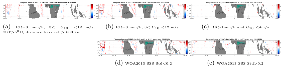
Figure 14: Temporal mean gridded over spatial boxes of size 1^\circ \times 1^\circ of \Delta SSS (SMAP SSS L3 v5.0 - 8-Day running (JPL) - TSG (SAMOS)) for 5 different subdatasets corresponding to: RR=0 mm/h, 3 < U_{10} < 12 m/s, SST>5°C, distance to coast > 800 km (a), RR=0 mm/h, 3 < U_{10} < 12 m/s (b), RR>1mm/h and U_{10} < 4 m/s (c), WOA2013 SSS Std<0.2 (d), WOA2013 SSS Std>0.2 (e).
