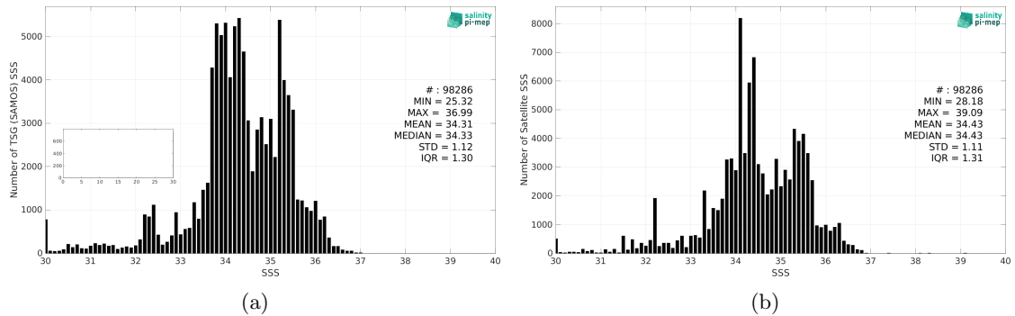
Figure 2: Histograms of SSS from TSG (SAMOS) (a) and SMAP SSS L3 v5.0 - 8-Day running (JPL) (b) considering all match-up pairs per bins of 0.1 over the Equatorial Ocean 10N-10S Pi-MEP region and for the full satellite product period.
