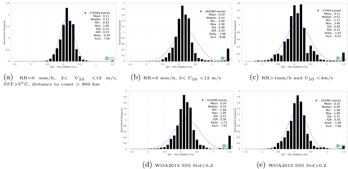
Figure 13: Normalized histogram of \Delta SSS (SMAP SSS L3 v5.0 - 8-Day running (JPL) - TSG (SAMOS)) for 5 different subdatasets corresponding to: RR=0 mm/h, 3 < U_{10} < 12 m/s, SST >5^\circ C, distance to coast > 800 km (a), RR=0 mm/h, 3 < U_{10} < 12 m/s (b), RR >1 mm/h and U_{10} < 4 m/s (c), WOA2013 SSS Std <0.2 (d), WOA2013 SSS Std >0.2 (e).
