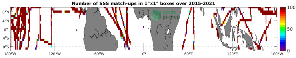
Figure 4: Number of SSS match-ups between TSG (SAMOS) SSS and the SMAP SSS L3 v5.0 - 8-Day running (JPL) SSS product for the Equatorial Ocean 10N-10S Pi-MEP region over 1^\circ \times 1^\circ boxes and for the full satellite product period.
