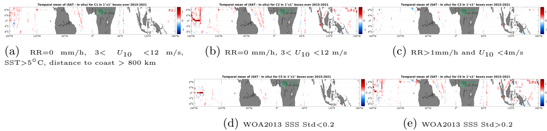
Figure 12: Temporal mean gridded over spatial boxes of size 1^\circ \times 1^\circ of \Delta SSS (SMAP SSS L3 v5.0 - 8-Day running (JPL) - TSG (SAMOS)) for 5 different subdatasets corresponding to: RR=0 mm/h, 3 < U_{10} < 12 m/s, SST>5°C, distance to coast > 800 km (a), RR=0 mm/h, 3 < U_{10} < 12 m/s (b), RR>1mm/h and U_{10} < 4 m/s (c), WOA2013 SSS Std<0.2 (d), WOA2013 SSS Std>0.2 (e).
