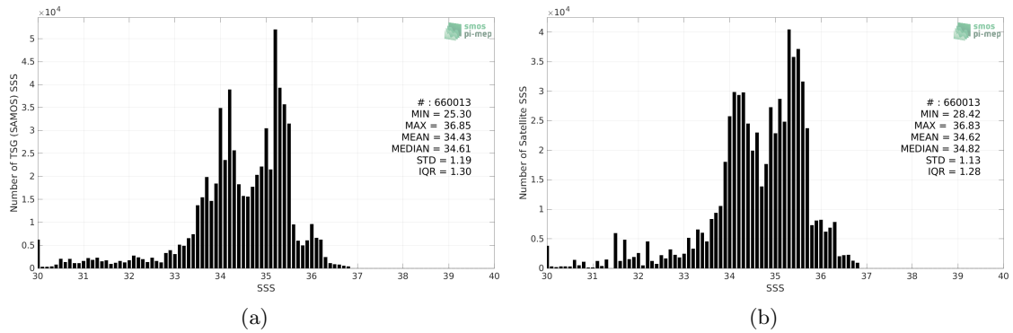
Figure 2: Histograms of SSS from TSG (SAMOS) (a) and SMAP SSS L3 v5.0 - 8-Day running (JPL) (b) considering all match-up pairs per bins of 0.1 over the Equatorial Ocean 10N-10S Pi-MEP region and for the full satellite product period.
