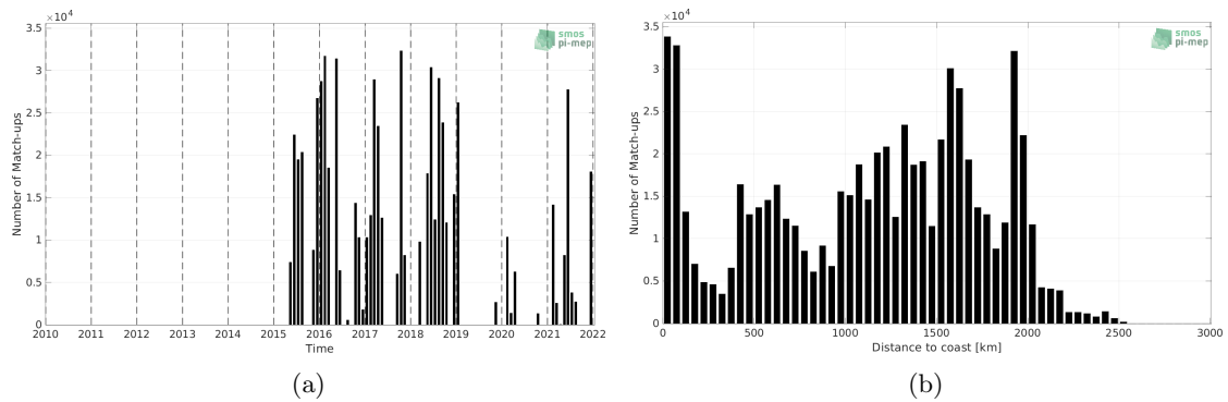
Figure 1: Number of match-ups between TSG (SAMOS) and SMAP SSS L3 v5.0 - 8-Day running (JPL) SSS as a function of time (a) and as function of the distance to coast (b) over the Equatorial Ocean 10N-10S Pi-MEP region and for the full satellite product period.
