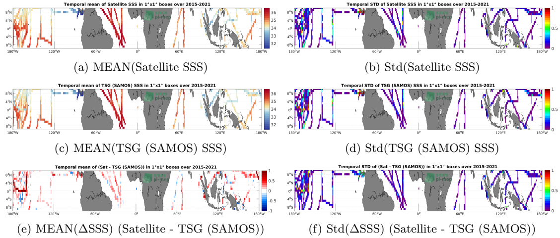
Figure 6: Temporal mean (left) and Std (right) of SSS from SMAP SSS L3 v5.0 - 8-Day running (JPL) (top), TSG (SAMOS) (middle), and of \Delta SSS (Satellite - TSG (SAMOS)). Only match-up pairs are used to generate these maps.
