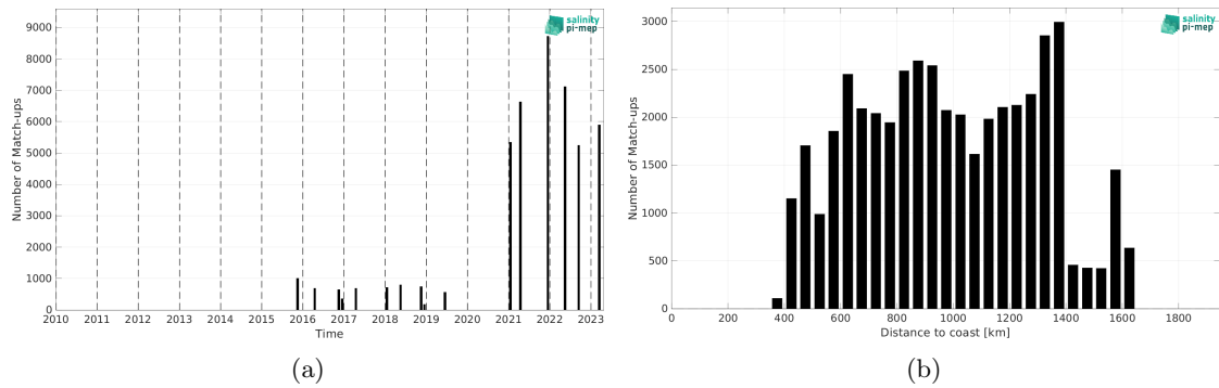
Figure 2: Number of match-ups between TSG (Polarstern) and SMAP SSS L3 v5.0 - 8-Day running (JPL) SSS as a function of time (a) and as function of the distance to coast (b) over the Equatorial Ocean 10N-10S Pi-MEP region and for the full satellite product period.
