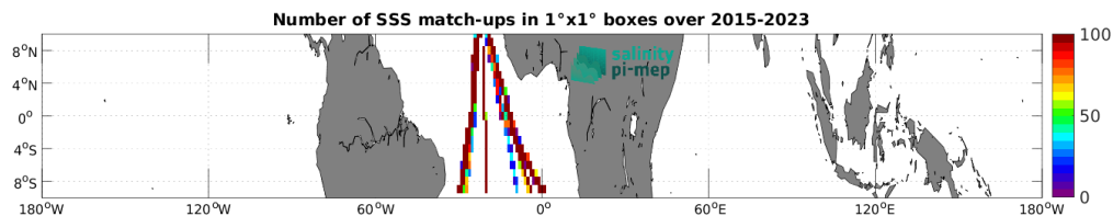
Figure 5: Number of SSS match-ups between TSG (Polarstern) SSS and the SMAP SSS L3 v5.0 - 8-Day running (JPL) SSS product for the Equatorial Ocean 10N-10S Pi-MEP region over 1^\circ \times 1^\circ boxes and for the full satellite product period.
