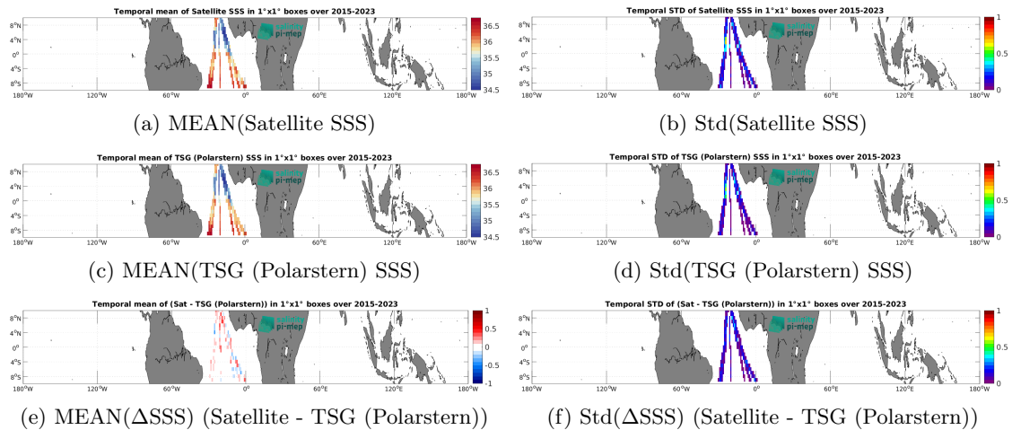
Figure 7: Temporal mean (left) and Std (right) of SSS from SMAP SSS L3 v5.0 - 8-Day running (JPL) (top), TSG (Polarstern) (middle), and of \Delta SSS (Satellite - TSG (Polarstern)). Only match-up pairs are used to generate these maps.
