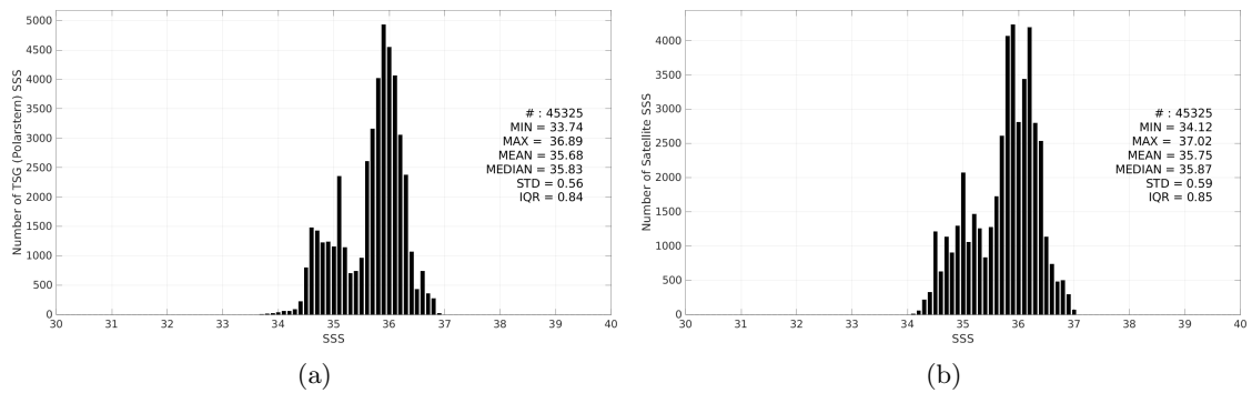
Figure 3: Histograms of SSS from TSG (Polarstern) (a) and SMAP SSS L3 v5.0 - 8-Day running (JPL) (b) considering all match-up pairs per bins of 0.1 over the Equatorial Ocean 10N-10S Pi-MEP region and for the full satellite product period.
