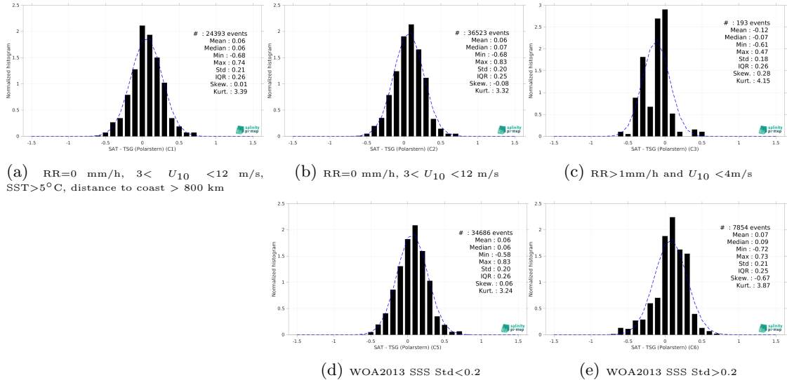
Figure 15: Normalized histogram of \Delta\text{SSS} (SMAP SSS L3 v5.0 - 8-Day running (JPL) - TSG (Polarstern)) for 5 different subdatasets corresponding to: RR=0 mm/h, 3 < U_{10} < 12 m/s, SST>5°C, distance to coast > 800 km (a), RR=0 mm/h, 3 < U_{10} < 12 m/s (b), RR>1mm/h and U_{10} < 4 m/s (c), WOA2013 SSS Std<0.2 (d), WOA2013 SSS Std>0.2 (e).
