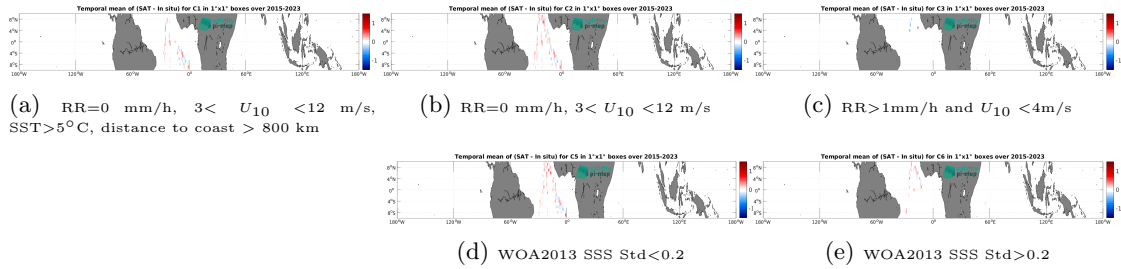
Figure 14: Temporal mean gridded over spatial boxes of size 1^\circ \times 1^\circ of \Delta\text{SSS} (SMAP SSS L3 v5.0 - 8-Day running (JPL) - TSG (Polarstern)) for 5 different subdatasets corresponding to:RR=0 mm/h, 3 < U_{10} < 12 m/s, SST>5°C, distance to coast > 800 km (a), RR=0 mm/h, 3 < U_{10} < 12 m/s (b), RR>1mm/h and U_{10} < 4 m/s (c), WOA2013 SSS Std<0.2 (d), WOA2013 SSS Std>0.2 (e).
