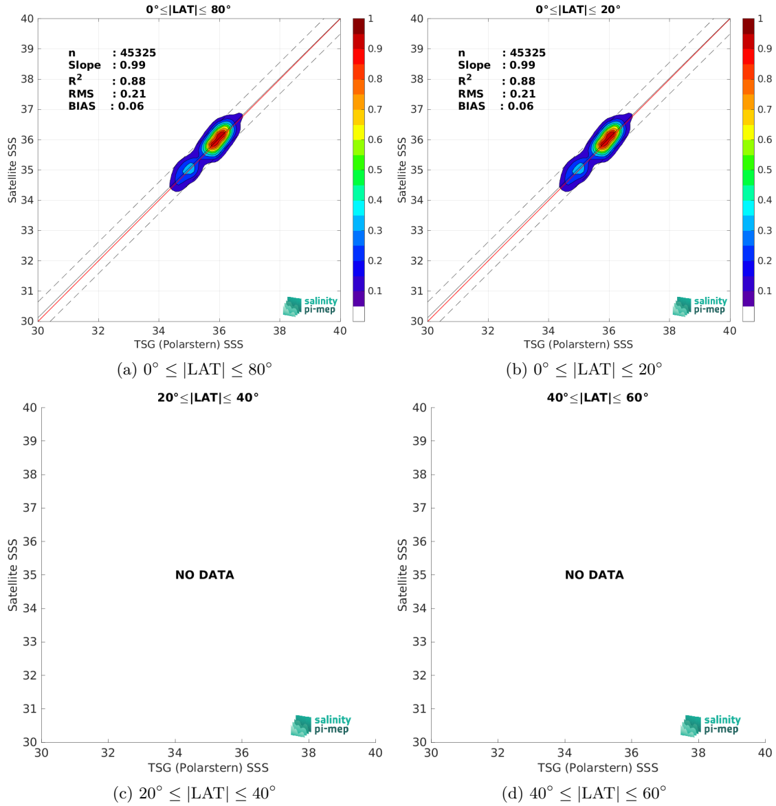
Figure 10: Contour maps of the concentration of SMAP SSS L3 v5.0 - 8-Day running (JPL) SSS (y-axis) versus TSG (Polarstern) SSS (x-axis) at match-up pairs for different latitude bands. For each plot, the red line shows x=y . The black thin and dashed lines indicate a linear fit through the data cloud and the \pm 95\% confidence levels, respectively. The number match-up pairs n , the slope and R^2 coefficient of the linear fit, the root mean square (RMS) and the mean bias between satellite and in situ data are indicated for each latitude band in each plots.
