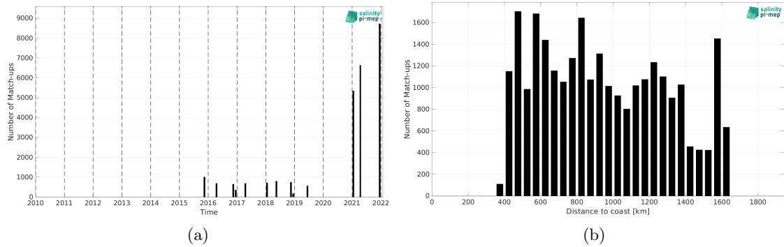
Figure 1: Number of match-ups between TSG (Polarstern) and SMAP SSS L3 v5.0 - 8-Day running (JPL) SSS as a function of time (a) and as function of the distance to coast (b) over the Equatorial Ocean 10N-10S Pi-MEP region and for the full satellite product period.
