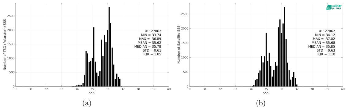
Figure 2: Histograms of SSS from TSG (Polarstern) (a) and SMAP SSS L3 v5.0 - 8-Day running (JPL) (b) considering all match-up pairs per bins of 0.1 over the Equatorial Ocean 10N-10S Pi-MEP region and for the full satellite product period.
