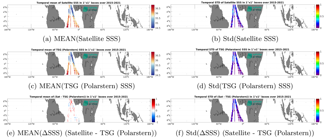
Figure 6: Temporal mean (left) and Std (right) of SSS from SMAP SSS L3 v5.0 - 8-Day running (JPL) (top), TSG (Polarstern) (middle), and of \Delta SSS (Satellite - TSG (Polarstern)). Only match-up pairs are used to generate these maps.
