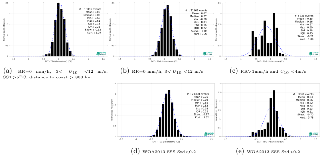
Figure 13: Normalized histogram of \Delta SSS (SMAP SSS L3 v5.0 - 8-Day running (JPL) - TSG (Polarstern)) for 5 different subdatasets corresponding to: RR=0 mm/h, 3 < U_{10} < 12 m/s, SST >5^\circ\text{C} , distance to coast > 800 km (a), RR=0 mm/h, 3 < U_{10} < 12 m/s (b), RR >1 mm/h and U_{10} < 4 m/s (c), WOA2013 SSS Std <0.2 (d), WOA2013 SSS Std >0.2 (e).
