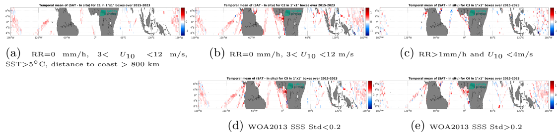
Figure 14: Temporal mean gridded over spatial boxes of size 1^\circ \times 1^\circ of \Delta SSS (SMAP SSS L3 v5.0 - 8-Day running (JPL) - TSG (LEGOS-DM)) for 5 different subdatasets corresponding to: RR=0 mm/h, 3 < U_{10} < 12 m/s, SST>5°C, distance to coast > 800 km (a), RR=0 mm/h, 3 < U_{10} < 12 m/s (b), RR>1mm/h and U_{10} < 4 m/s (c), WOA2013 SSS Std<0.2 (d), WOA2013 SSS Std>0.2 (e).
