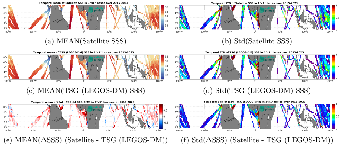
Figure 7: Temporal mean (left) and Std (right) of SSS from SMAP SSS L3 v5.0 - 8-Day running (JPL) (top), TSG (LEGOS-DM) (middle), and of \Delta SSS (Satellite - TSG (LEGOS-DM)). Only match-up pairs are used to generate these maps.
