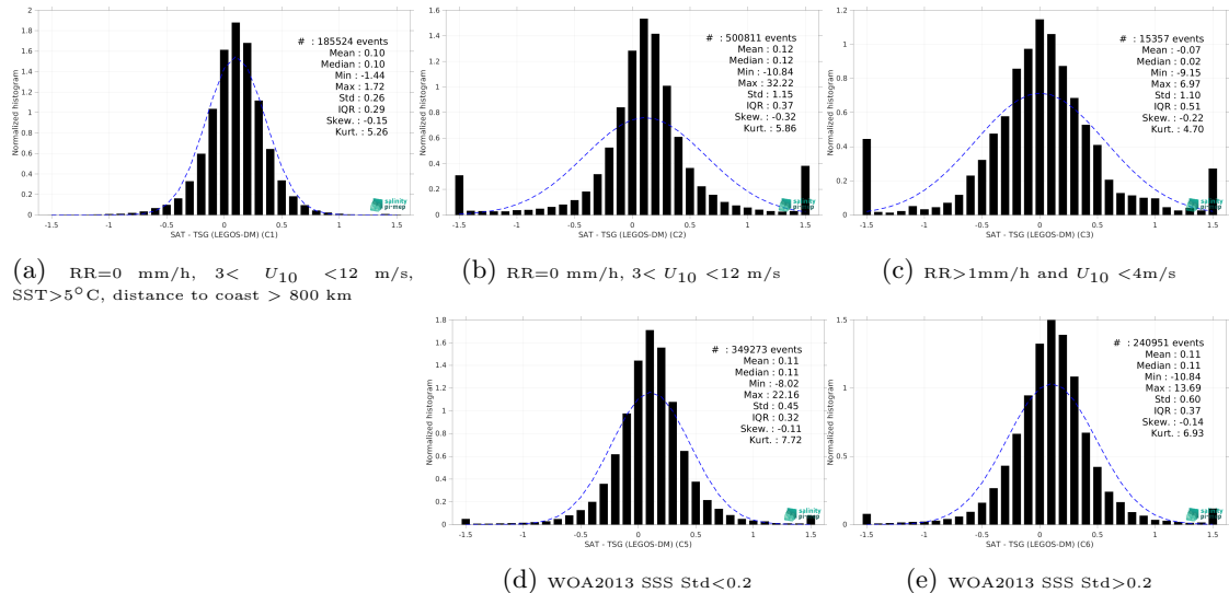
Figure 15: Normalized histogram of \Delta SSS (SMAP SSS L3 v5.0 - 8-Day running (JPL) - TSG (LEGOS-DM)) for 5 different subdatasets corresponding to: RR=0 mm/h, 3 < U_{10} < 12 m/s, SST>5°C, distance to coast > 800 km (a), RR=0 mm/h, 3 < U_{10} < 12 m/s (b), RR>1mm/h and U_{10} < 4 m/s (c), WOA2013 SSS Std<0.2 (d), WOA2013 SSS Std>0.2 (e).
