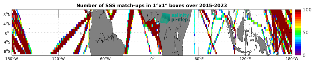
Figure 5: Number of SSS match-ups between TSG (LEGOS-DM) SSS and the SMAP SSS L3 v5.0 - 8-Day running (JPL) SSS product for the Equatorial Ocean 10N-10S Pi-MEP region over 1^\circ \times 1^\circ boxes and for the full satellite product period.
