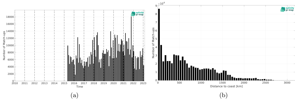
Figure 2: Number of match-ups between TSG (LEGOS-DM) and SMAP SSS L3 v5.0 - 8-Day running (JPL) SSS as a function of time (a) and as function of the distance to coast (b) over the Equatorial Ocean 10N-10S Pi-MEP region and for the full satellite product period.
