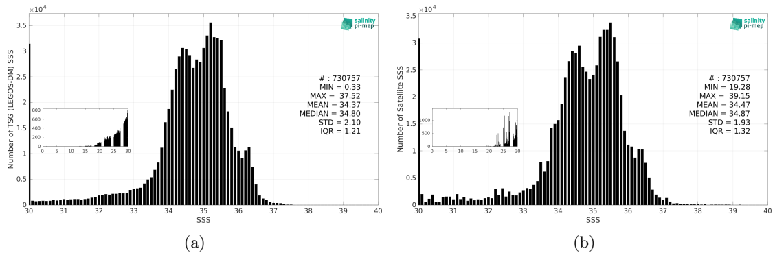
Figure 3: Histograms of SSS from TSG (LEGOS-DM) (a) and SMAP SSS L3 v5.0 - 8-Day running (JPL) (b) considering all match-up pairs per bins of 0.1 over the Equatorial Ocean 10N-10S Pi-MEP region and for the full satellite product period.
