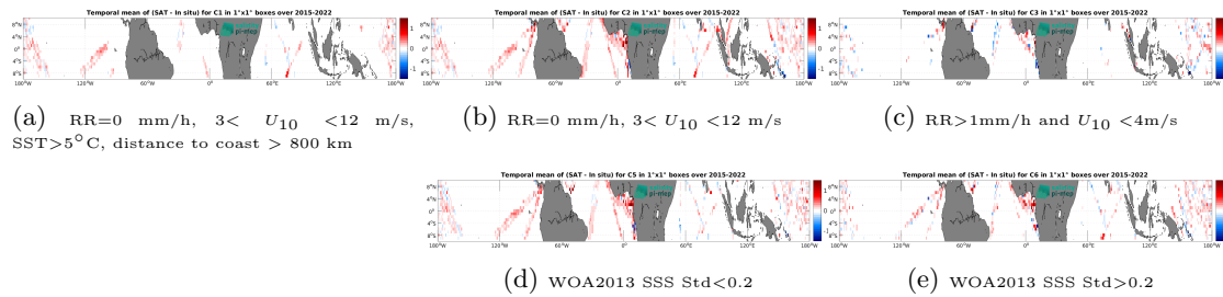
Figure 12: Temporal mean gridded over spatial boxes of size 1^\circ \times 1^\circ of \Delta\text{SSS} (SMAP SSS L3 v5.0 - 8-Day running (JPL) - TSG (LEGOS-DM)) for 5 different subdatasets corresponding to: RR=0 mm/h, 3 < U_{10} < 12 m/s, SST >5^\circ\text{C} , distance to coast > 800 km (a), RR=0 mm/h, 3 < U_{10} < 12 m/s (b), RR >1 mm/h and U_{10} < 4 m/s (c), WOA2013 SSS Std <0.2 (d), WOA2013 SSS Std >0.2 (e).
