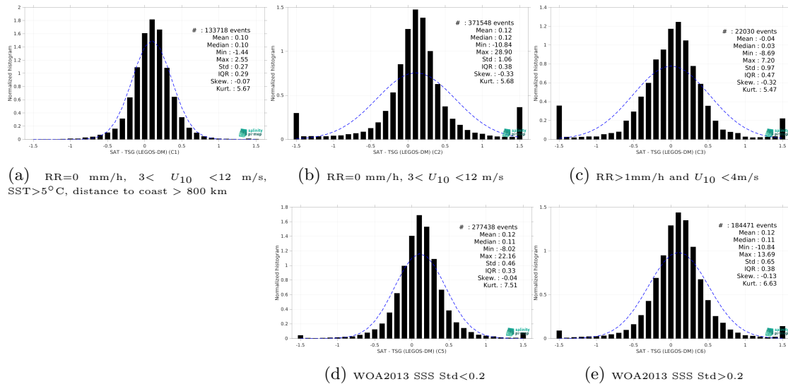
Figure 13: Normalized histogram of \Delta\text{SSS} (SMAP SSS L3 v5.0 - 8-Day running (JPL) - TSG (LEGOS-DM)) for 5 different subdatasets corresponding to: RR=0 mm/h, 3 < U_{10} < 12 m/s, SST >5^\circ\text{C} , distance to coast > 800 km (a), RR=0 mm/h, 3 < U_{10} < 12 m/s (b), RR >1 mm/h and U_{10} < 4 m/s (c), WOA2013 SSS Std <0.2 (d), WOA2013 SSS Std >0.2 (e).
