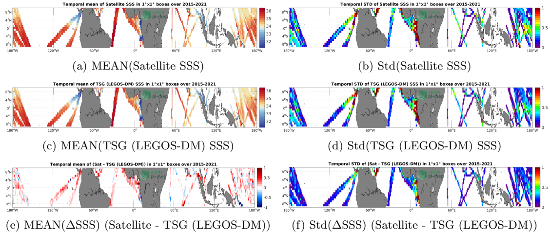
Figure 6: Temporal mean (left) and Std (right) of SSS from SMAP SSS L3 v5.0 - 8-Day running (JPL) (top), TSG (LEGOS-DM) (middle), and of \Delta SSS (Satellite - TSG (LEGOS-DM)). Only match-up pairs are used to generate these maps.
