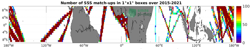
Figure 4: Number of SSS match-ups between TSG (LEGOS-DM) SSS and the SMAP SSS L3 v5.0 - 8-Day running (JPL) SSS product for the Equatorial Ocean 10N-10S Pi-MEP region over 1^\circ \times 1^\circ boxes and for the full satellite product period.
