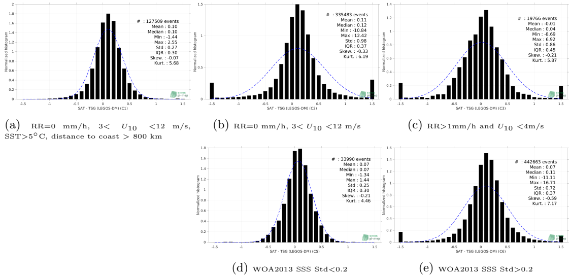
Figure 13: Normalized histogram of \Delta SSS (SMAP SSS L3 v5.0 - 8-Day running (JPL) - TSG (LEGOS-DM)) for 5 different subdatasets corresponding to: RR=0 mm/h, 3 < U_{10} < 12 m/s, SST >5^\circ\text{C} , distance to coast > 800 km (a), RR=0 mm/h, 3 < U_{10} < 12 m/s (b), RR >1 mm/h and U_{10} < 4 m/s (c), WOA2013 SSS Std <0.2 (d), WOA2013 SSS Std >0.2 (e).
