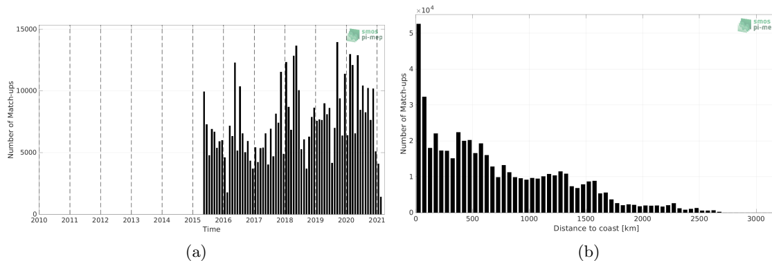
Figure 1: Number of match-ups between TSG (LEGOS-DM) and SMAP SSS L3 v5.0 - 8-Day running (JPL) SSS as a function of time (a) and as function of the distance to coast (b) over the Equatorial Ocean 10N-10S Pi-MEP region and for the full satellite product period.
