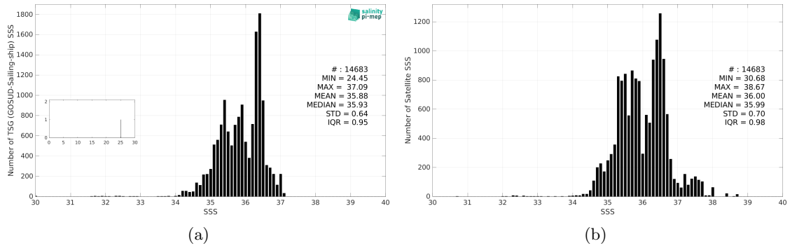
Figure 3: Histograms of SSS from TSG (GOSUD-Sailing-ship) (a) and SMAP SSS L3 v5.0 - 8-Day running (JPL) (b) considering all match-up pairs per bins of 0.1 over the Equatorial Ocean 10N-10S Pi-MEP region and for the full satellite product period.
