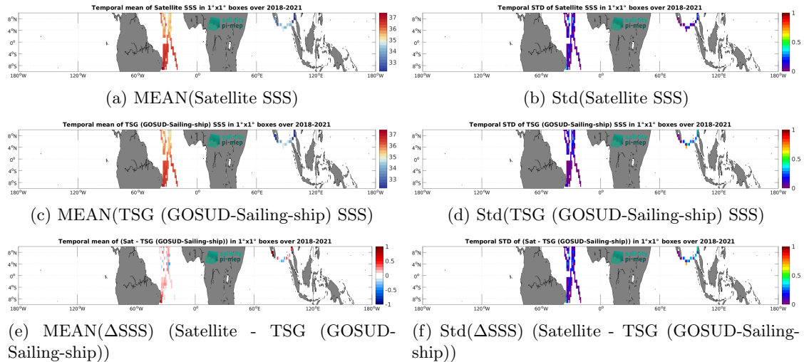
Figure 7: Temporal mean (left) and Std (right) of SSS from SMAP SSS L3 v5.0 - 8-Day running (JPL) (top), TSG (GOSUD-Sailing-ship) (middle), and of \Delta SSS (Satellite - TSG (GOSUD-Sailing-ship)). Only match-up pairs are used to generate these maps.
