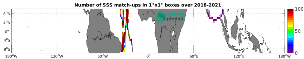
Figure 5: Number of SSS match-ups between TSG (GOSUD-Sailing-ship) SSS and the SMAP SSS L3 v5.0 - 8-Day running (JPL) SSS product for the Equatorial Ocean 10N-10S Pi-MEP region over 1^\circ \times 1^\circ boxes and for the full satellite product period.
