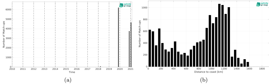
Figure 2: Number of match-ups between TSG (GOSUD-Sailing-ship) and SMAP SSS L3 v5.0 - 8-Day running (JPL) SSS as a function of time (a) and as function of the distance to coast (b) over the Equatorial Ocean 10N-10S Pi-MEP region and for the full satellite product period.
