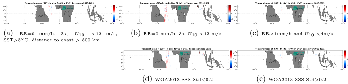
Figure 14: Temporal mean gridded over spatial boxes of size 1^\circ \times 1^\circ of \Delta SSS (SMAP SSS L3 v5.0 - 8-Day running (JPL) - TSG (GOSUD-Sailing-ship)) for 5 different subdatasets corresponding to: RR=0 mm/h, 3 < U_{10} < 12 m/s, SST>5°C, distance to coast > 800 km (a), RR=0 mm/h, 3 < U_{10} < 12 m/s (b), RR>1mm/h and U_{10} < 4 m/s (c), WOA2013 SSS Std<0.2 (d), WOA2013 SSS Std>0.2 (e).
