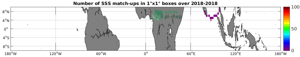
Figure 4: Number of SSS match-ups between TSG (GOSUD-Sailing-ship) SSS and the SMAP SSS L3 v5.0 - 8-Day running (JPL) SSS product for the Equatorial Ocean 10N-10S Pi-MEP region over 1°x1° boxes and for the full satellite product period.
