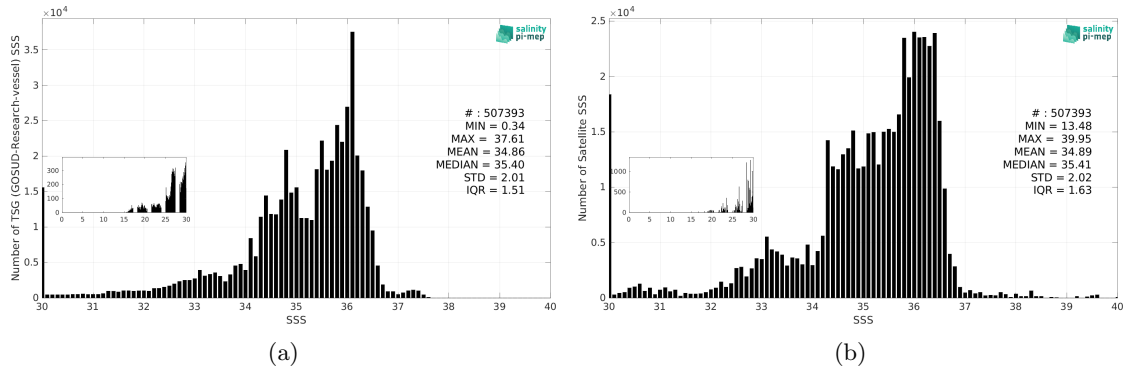
Figure 3: Histograms of SSS from TSG (GOSUD-Research-vessel) (a) and SMAP SSS L3 v5.0 - 8-Day running (JPL) (b) considering all match-up pairs per bins of 0.1 over the Equatorial Ocean 10N-10S Pi-MEP region and for the full satellite product period.
