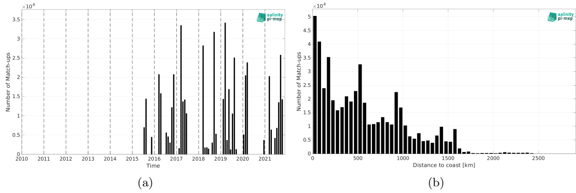
Figure 2: Number of match-ups between TSG (GOSUD-Research-vessel) and SMAP SSS L3 v5.0 - 8-Day running (JPL) SSS as a function of time (a) and as function of the distance to coast (b) over the Equatorial Ocean 10N-10S Pi-MEP region and for the full satellite product period.
