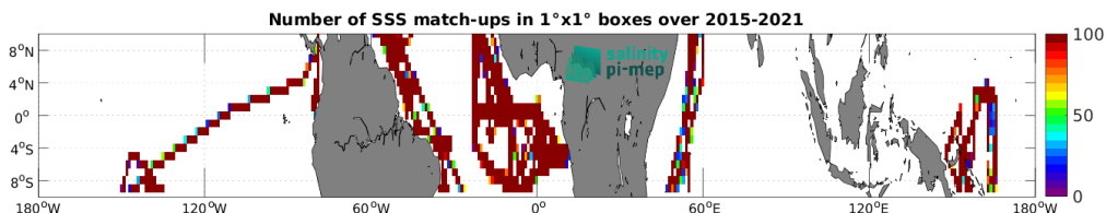
Figure 5: Number of SSS match-ups between TSG (GOSUD-Research-vessel) SSS and the SMAP SSS L3 v5.0 - 8-Day running (JPL) SSS product for the Equatorial Ocean 10N-10S Pi-MEP region over 1^\circ \times 1^\circ boxes and for the full satellite product period.
