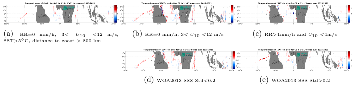
Figure 14: Temporal mean gridded over spatial boxes of size 1^\circ \times 1^\circ of \Delta SSS (SMAP SSS L3 v5.0 - 8-Day running (JPL) - TSG (GOSUD-Research-vessel)) for 5 different subdatasets corresponding to:RR=0 mm/h, 3 < U_{10} < 12 m/s, SST>5°C, distance to coast > 800 km (a), RR=0 mm/h, 3 < U_{10} < 12 m/s (b), RR>1mm/h and U_{10} < 4 m/s (c), WOA2013 SSS Std<0.2 (d), WOA2013 SSS Std>0.2 (e).
