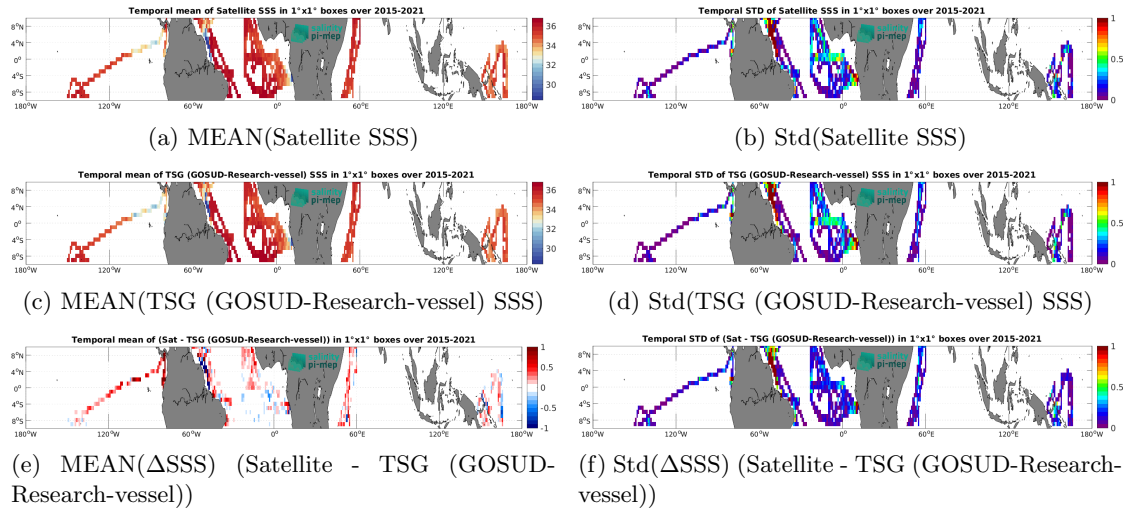
Figure 7: Temporal mean (left) and Std (right) of SSS from SMAP SSS L3 v5.0 - 8-Day running (JPL) (top), TSG (GOSUD-Research-vessel) (middle), and of \Delta SSS (Satellite - TSG (GOSUD-Research-vessel)). Only match-up pairs are used to generate these maps.
