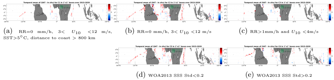
Figure 12: Temporal mean gridded over spatial boxes of size 1^{\circ}\times 1^{\circ} of \Delta SSS (SMAP SSS L3 v5.0 - 8-Day running (JPL) - TSG (GOSUD-Research-vessel)) for 5 different subdatasets corresponding to:RR=0 mm/h, 3 < U_{10} < 12 m/s, SST >5^{\circ}\text{C} , distance to coast > 800 km (a), RR=0 mm/h, 3 < U_{10} < 12 m/s (b), RR >1 mm/h and U_{10} < 4 m/s (c), WOA2013 SSS Std <0.2 (d), WOA2013 SSS Std >0.2 (e).
