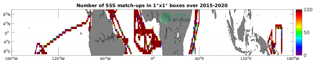
Figure 4: Number of SSS match-ups between TSG (GOSUD-Research-vessel) SSS and the SMAP SSS L3 v5.0 - 8-Day running (JPL) SSS product for the Equatorial Ocean 10N-10S Pi-MEP region over 1^\circ \times 1^\circ boxes and for the full satellite product period.
