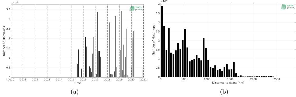
Figure 1: Number of match-ups between TSG (GOSUD-Research-vessel) and SMAP SSS L3 v5.0 - 8-Day running (JPL) SSS as a function of time (a) and as function of the distance to coast (b) over the Equatorial Ocean 10N-10S Pi-MEP region and for the full satellite product period.
