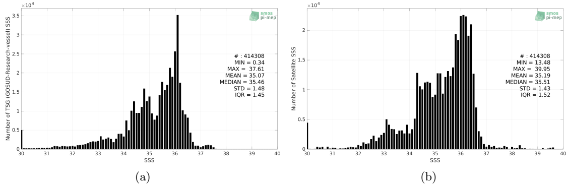
Figure 2: Histograms of SSS from TSG (GOSUD-Research-vessel) (a) and SMAP SSS L3 v5.0 - 8-Day running (JPL) (b) considering all match-up pairs per bins of 0.1 over the Equatorial Ocean 10N-10S Pi-MEP region and for the full satellite product period.
