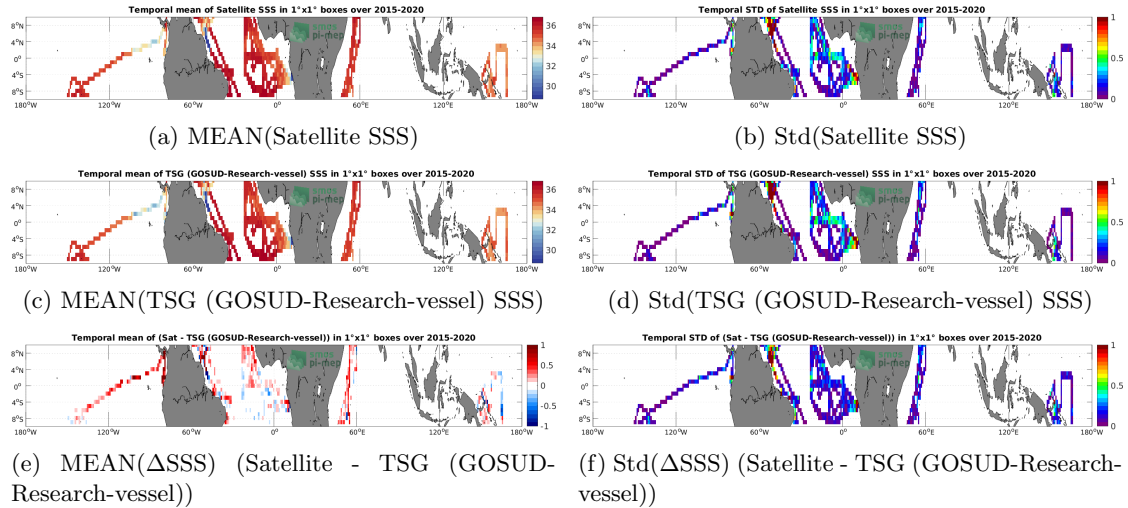
Figure 6: Temporal mean (left) and Std (right) of SSS from SMAP SSS L3 v5.0 - 8-Day running (JPL) (top), TSG (GOSUD-Research-vessel) (middle), and of \Delta SSS (Satellite - TSG (GOSUD-Research-vessel)). Only match-up pairs are used to generate these maps.
