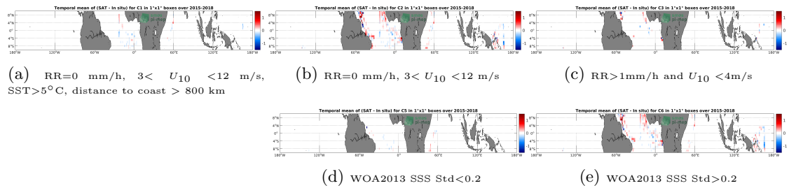
Figure 12: Temporal mean gridded over spatial boxes of size 1^\circ \times 1^\circ of \Delta SSS (SMAP SSS L3 v5.0 - 8-Day running (JPL) - TSG (GOSUD-Research-vessel)) for 5 different subdatasets corresponding to: RR=0 mm/h, 3 < U_{10} < 12 m/s, SST > 5^\circ\text{C} , distance to coast > 800 km (a), RR=0 mm/h, 3 < U_{10} < 12 m/s (b), RR > 1 mm/h and U_{10} < 4 m/s (c), WOA2013 SSS Std < 0.2 (d), WOA2013 SSS Std > 0.2 (e).
