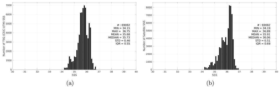
Figure 3: Histograms of SSS from TSG (CSIC-UTM) (a) and SMAP SSS L3 v5.0 - 8-Day running (JPL) (b) considering all match-up pairs per bins of 0.1 over the Equatorial Ocean 10N-10S Pi-MEP region and for the full satellite product period.
