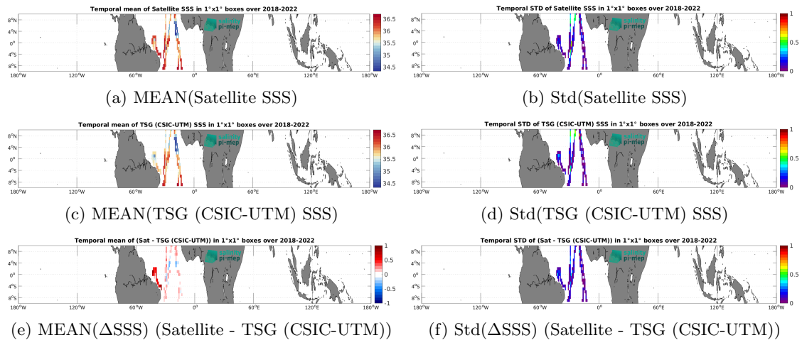
Figure 7: Temporal mean (left) and Std (right) of SSS from SMAP SSS L3 v5.0 - 8-Day running (JPL) (top), TSG (CSIC-UTM) (middle), and of \Delta SSS (Satellite - TSG (CSIC-UTM)). Only match-up pairs are used to generate these maps.
