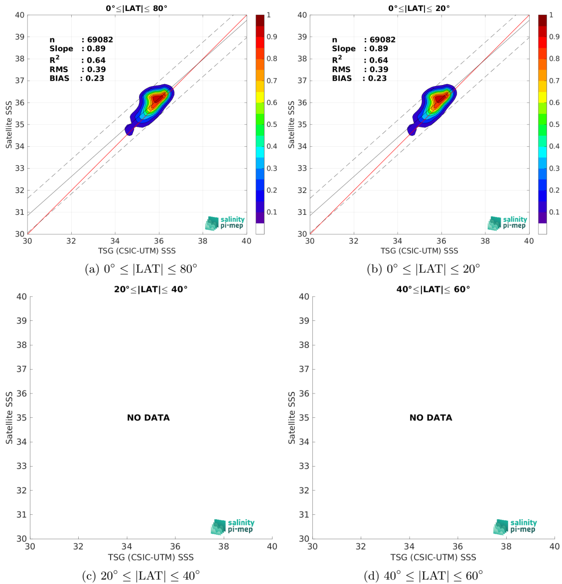
Figure 10: Contour maps of the concentration of SMAP SSS L3 v5.0 - 8-Day running (JPL) SSS (y-axis) versus TSG (CSIC-UTM) SSS (x-axis) at match-up pairs for different latitude bands. For each plot, the red line shows x=y . The black thin and dashed lines indicate a linear fit through the data cloud and the \pm 95\% confidence levels, respectively. The number match-up pairs n , the slope and R^2 coefficient of the linear fit, the root mean square (RMS) and the mean bias between satellite and in situ data are indicated for each latitude band in each plots.
