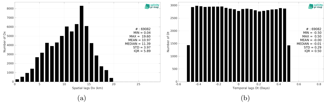
Figure 6: Histograms of the spatial (a) and temporal (b) lags between the location/time of the TSG (CSIC-UTM) measurement and the date of the corresponding SMAP SSS L3 v5.0 - 8-Day running (JPL) SSS pixel.
