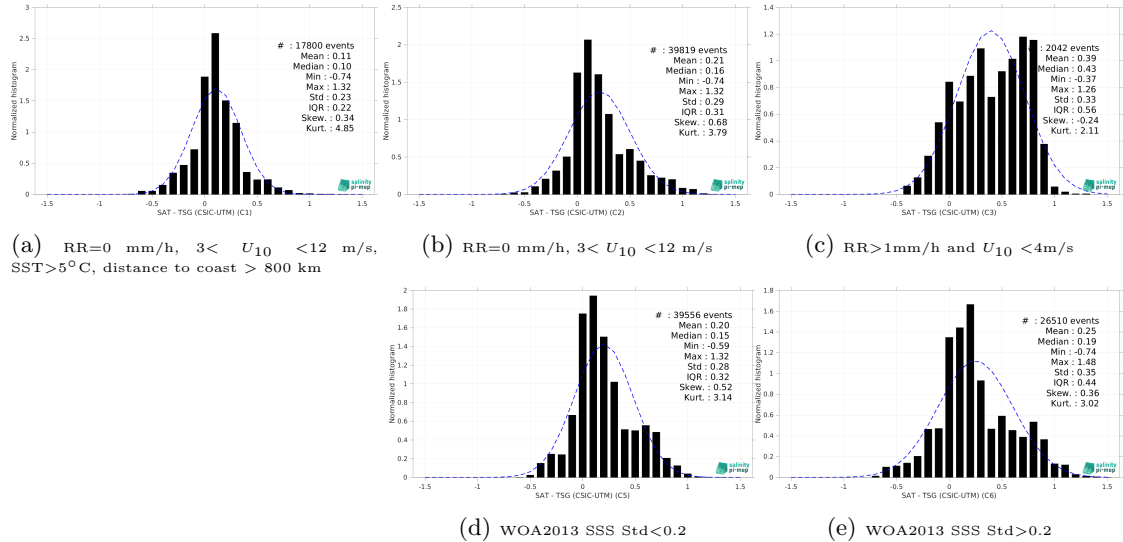
Figure 15: Normalized histogram of \Delta SSS (SMAP SSS L3 v5.0 - 8-Day running (JPL) - TSG (CSIC-UTM)) for 5 different subdatasets corresponding to: RR=0 mm/h, 3 < U_{10} < 12 m/s, SST>5°C, distance to coast > 800 km (a), RR=0 mm/h, 3 < U_{10} < 12 m/s (b), RR>1mm/h and U_{10} < 4 m/s (c), WOA2013 SSS Std<0.2 (d), WOA2013 SSS Std>0.2 (e).
