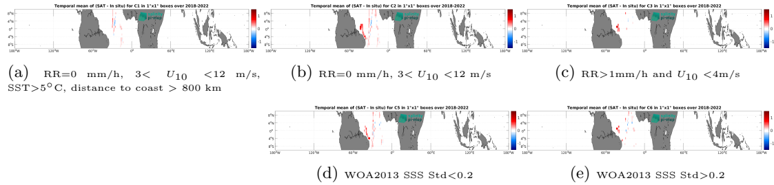
Figure 14: Temporal mean gridded over spatial boxes of size 1^\circ \times 1^\circ of \Delta SSS (SMAP SSS L3 v5.0 - 8-Day running (JPL) - TSG (CSIC-UTM)) for 5 different subdatasets corresponding to: RR=0 mm/h, 3 < U_{10} < 12 m/s, SST>5°C, distance to coast > 800 km (a), RR=0 mm/h, 3 < U_{10} < 12 m/s (b), RR>1mm/h and U_{10} < 4 m/s (c), WOA2013 SSS Std<0.2 (d), WOA2013 SSS Std>0.2 (e).
