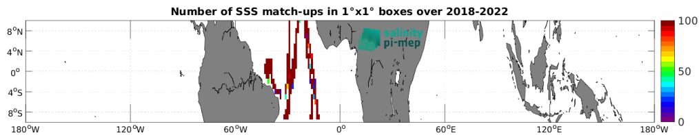
Figure 5: Number of SSS match-ups between TSG (CSIC-UTM) SSS and the SMAP SSS L3 v5.0 - 8-Day running (JPL) SSS product for the Equatorial Ocean 10N-10S Pi-MEP region over 1^\circ \times 1^\circ boxes and for the full satellite product period.
