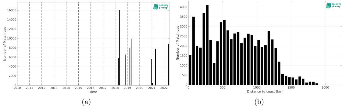
Figure 2: Number of match-ups between TSG (CSIC-UTM) and SMAP SSS L3 v5.0 - 8-Day running (JPL) SSS as a function of time (a) and as function of the distance to coast (b) over the Equatorial Ocean 10N-10S Pi-MEP region and for the full satellite product period.
