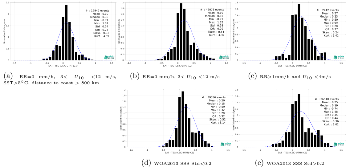
Figure 13: Normalized histogram of \Delta SSS (SMAP SSS L3 v5.0 - 8-Day running (JPL) - TSG (CSIC-UTM)) for 5 different subdatasets corresponding to: RR=0 mm/h, 3 < U_{10} < 12 m/s, SST >5^\circ C, distance to coast > 800 km (a), RR=0 mm/h, 3 < U_{10} < 12 m/s (b), RR >1 mm/h and U_{10} < 4 m/s (c), WOA2013 SSS Std <0.2 (d), WOA2013 SSS Std >0.2 (e).
