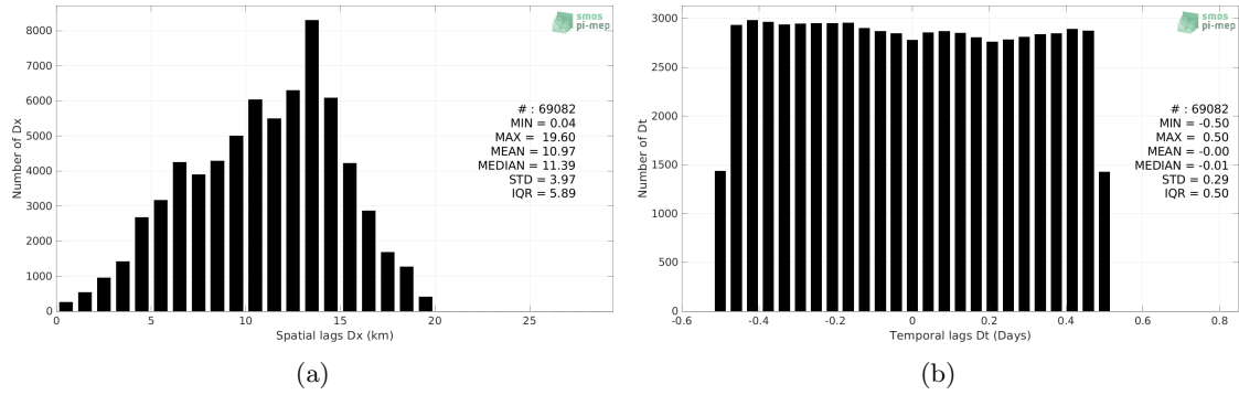
Figure 5: Histograms of the spatial (a) and temporal (b) lags between the location/time of the TSG (CSIC-UTM) measurement and the date of the corresponding SMAP SSS L3 v5.0 - 8-Day running (JPL) SSS pixel.
