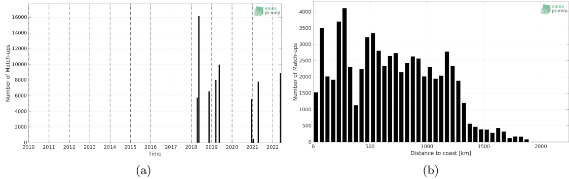
Figure 1: Number of match-ups between TSG (CSIC-UTM) and SMAP SSS L3 v5.0 - 8-Day running (JPL) SSS as a function of time (a) and as function of the distance to coast (b) over the Equatorial Ocean 10N-10S Pi-MEP region and for the full satellite product period.
