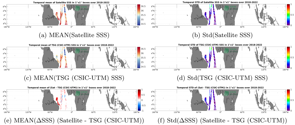
Figure 6: Temporal mean (left) and Std (right) of SSS from SMAP SSS L3 v5.0 - 8-Day running (JPL) (top), TSG (CSIC-UTM) (middle), and of \Delta SSS (Satellite - TSG (CSIC-UTM)). Only match-up pairs are used to generate these maps.
