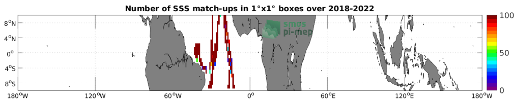
Figure 4: Number of SSS match-ups between TSG (CSIC-UTM) SSS and the SMAP SSS L3 v5.0 - 8-Day running (JPL) SSS product for the Equatorial Ocean 10N-10S Pi-MEP region over 1^\circ \times 1^\circ boxes and for the full satellite product period.
