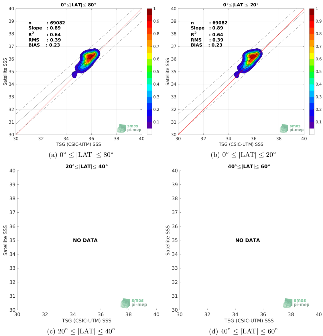
Figure 9: Contour maps of the concentration of SMAP SSS L3 v5.0 - 8-Day running (JPL) SSS (y-axis) versus TSG (CSIC-UTM) SSS (x-axis) at match-up pairs for different latitude bands. For each plot, the red line shows x=y . The black thin and dashed lines indicate a linear fit through the data cloud and the \pm 95\% confidence levels, respectively. The number match-up pairs n , the slope and R^2 coefficient of the linear fit, the root mean square (RMS) and the mean bias between satellite and in situ data are indicated for each latitude band in each plots.
