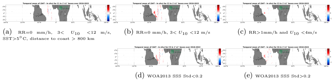
Figure 12: Temporal mean gridded over spatial boxes of size 1^\circ \times 1^\circ of \Delta SSS (SMAP SSS L3 v5.0 - 8-Day running (JPL) - TSG (CSIC-UTM)) for 5 different subdatasets corresponding to: RR=0 mm/h, 3 < U_{10} < 12 m/s, SST>5°C, distance to coast > 800 km (a), RR=0 mm/h, 3 < U_{10} < 12 m/s (b), RR>1mm/h and U_{10} < 4 m/s (c), WOA2013 SSS Std<0.2 (d), WOA2013 SSS Std>0.2 (e).
