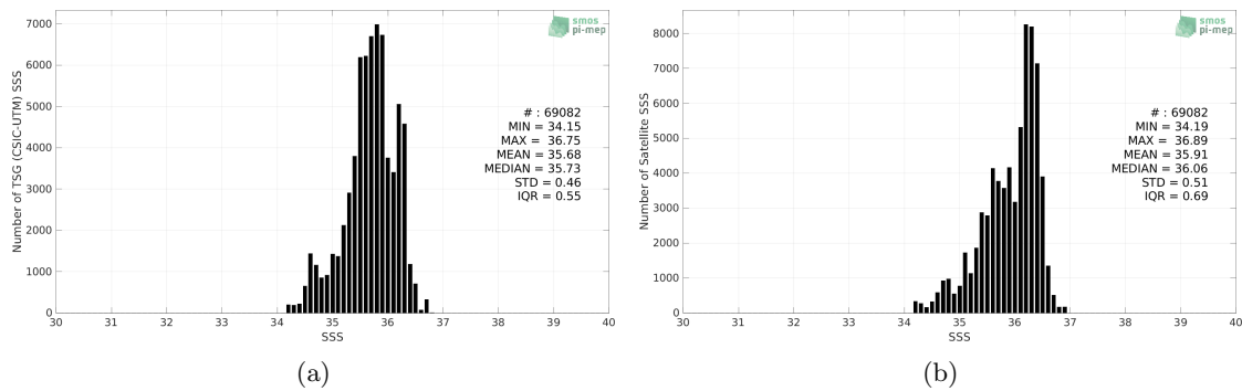
Figure 2: Histograms of SSS from TSG (CSIC-UTM) (a) and SMAP SSS L3 v5.0 - 8-Day running (JPL) (b) considering all match-up pairs per bins of 0.1 over the Equatorial Ocean 10N-10S Pi-MEP region and for the full satellite product period.
