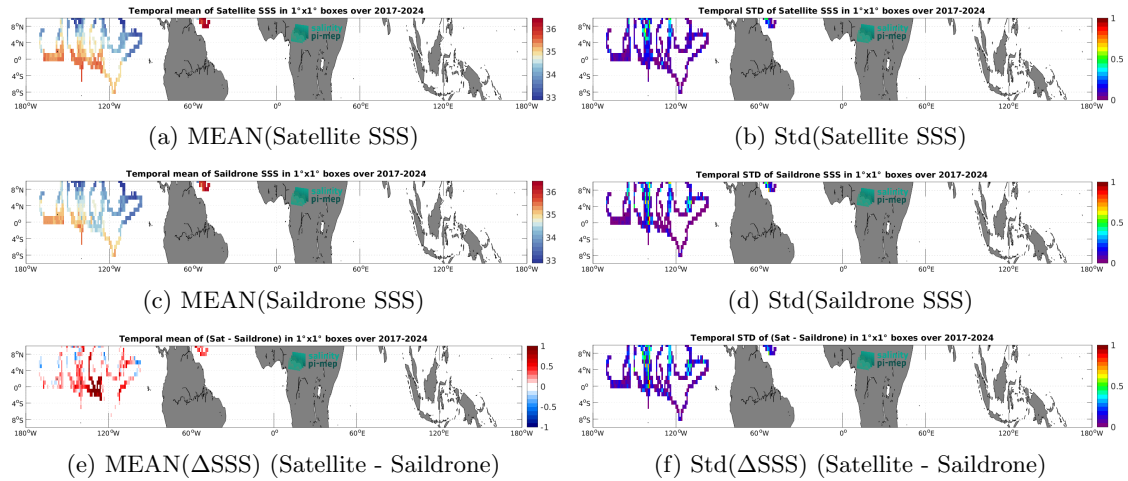
Figure 7: Temporal mean (left) and Std (right) of SSS from SMAP SSS L3 v5.0 - 8-Day running (JPL) (top), Saildrone (middle), and of \Delta SSS (Satellite - Saildrone). Only match-up pairs are used to generate these maps.
