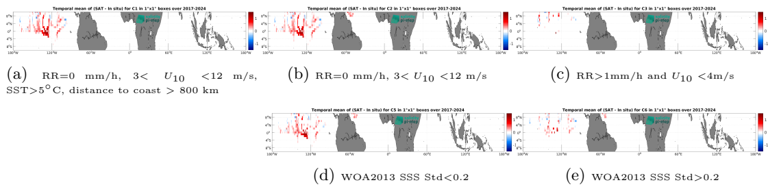
Figure 14: Temporal mean gridded over spatial boxes of size 1^\circ \times 1^\circ of \Delta\text{SSS} (SMAP SSS L3 v5.0 - 8-Day running (JPL) - Saildrone) for 5 different subdatasets corresponding to:RR=0 mm/h, 3 < U_{10} < 12 m/s, SST>5°C, distance to coast > 800 km (a), RR=0 mm/h, 3 < U_{10} < 12 m/s (b), RR>1mm/h and U_{10} < 4 m/s (c), WOA2013 SSS Std<0.2 (d), WOA2013 SSS Std>0.2 (e).
