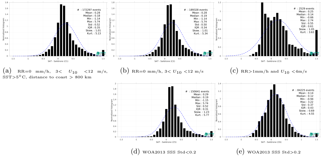
Figure 15: Normalized histogram of \Delta\text{SSS} (SMAP SSS L3 v5.0 - 8-Day running (JPL) - Saildrone) for 5 different subdatasets corresponding to: RR=0 mm/h, 3 < U_{10} < 12 m/s, SST>5°C, distance to coast > 800 km (a), RR=0 mm/h, 3 < U_{10} < 12 m/s (b), RR>1mm/h and U_{10} < 4 m/s (c), WOA2013 SSS Std<0.2 (d), WOA2013 SSS Std>0.2 (e).
