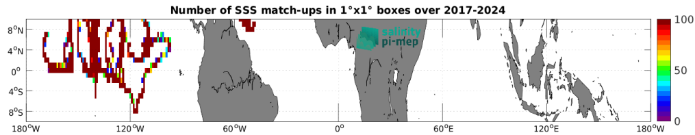
Figure 5: Number of SSS match-ups between Saildrone SSS and the SMAP SSS L3 v5.0 - 8-Day running (JPL) SSS product for the Equatorial Ocean 10N-10S Pi-MEP region over 1^\circ \times 1^\circ boxes and for the full satellite product period.
