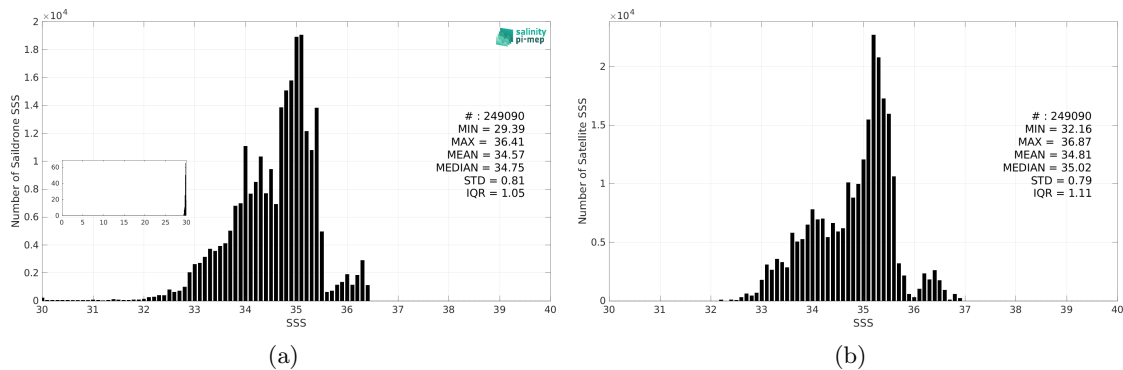
Figure 3: Histograms of SSS from Sairdrone (a) and SMAP SSS L3 v5.0 - 8-Day running (JPL) (b) considering all match-up pairs per bins of 0.1 over the Equatorial Ocean 10N-10S Pi-MEP region and for the full satellite product period.
