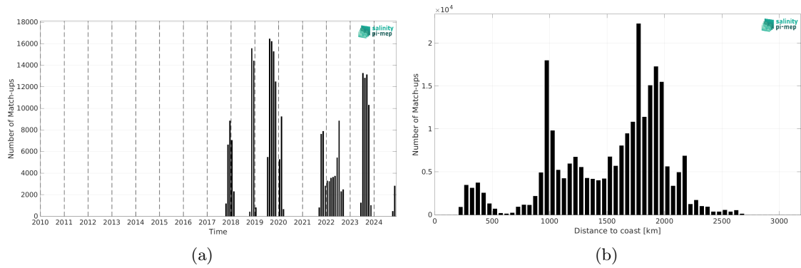
Figure 2: Number of match-ups between Sairdrone and SMAP SSS L3 v5.0 - 8-Day running (JPL) SSS as a function of time (a) and as function of the distance to coast (b) over the Equatorial Ocean 10N-10S Pi-MEP region and for the full satellite product period.
