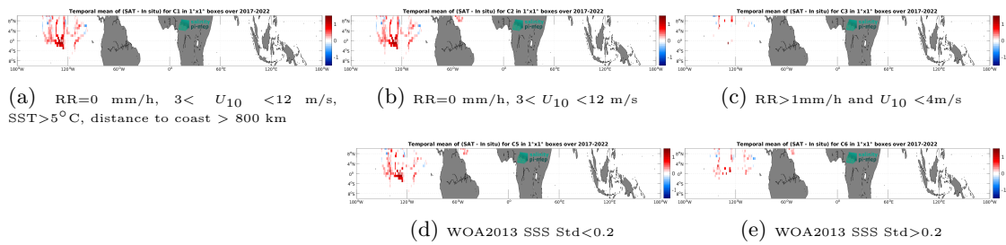
Figure 14: Temporal mean gridded over spatial boxes of size 1^\circ \times 1^\circ of \Delta SSS (SMAP SSS L3 v5.0 - 8-Day running (JPL) - Saildrone) for 5 different subdatasets corresponding to: RR=0 mm/h, 3 < U_{10} < 12 m/s, SST > 5°C, distance to coast > 800 km (a), RR=0 mm/h, 3 < U_{10} < 12 m/s (b), RR > 1mm/h and U_{10} < 4 m/s (c), WOA2013 SSS Std < 0.2 (d), WOA2013 SSS Std > 0.2 (e).
