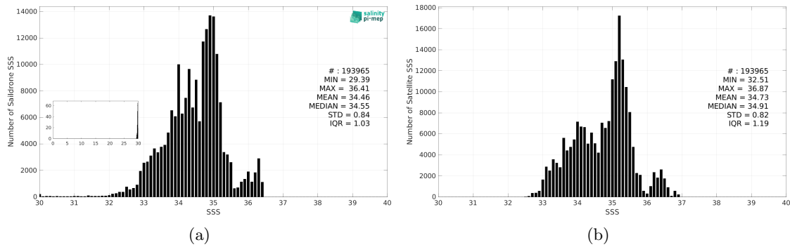
Figure 3: Histograms of SSS from Saildrone (a) and SMAP SSS L3 v5.0 - 8-Day running (JPL) (b) considering all match-up pairs per bins of 0.1 over the Equatorial Ocean 10N-10S Pi-MEP region and for the full satellite product period.
