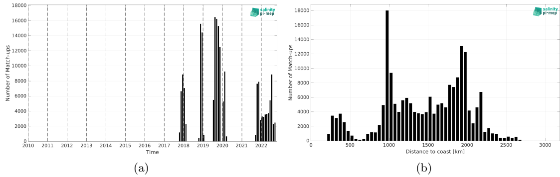
Figure 2: Number of match-ups between Saildrone and SMAP SSS L3 v5.0 - 8-Day running (JPL) SSS as a function of time (a) and as function of the distance to coast (b) over the Equatorial Ocean 10N-10S Pi-MEP region and for the full satellite product period.
