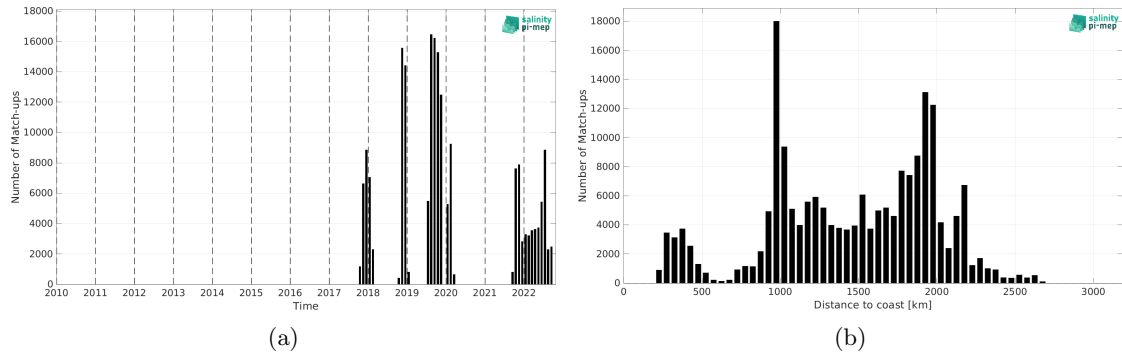
Figure 1: Number of match-ups between Saildrone and SMAP SSS L3 v5.0 - 8-Day running (JPL) SSS as a function of time (a) and as function of the distance to coast (b) over the Equatorial Ocean 10N-10S Pi-MEP region and for the full satellite product period.
