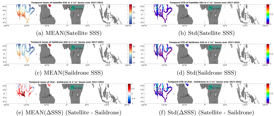
Figure 6: Temporal mean (left) and Std (right) of SSS from SMAP SSS L3 v5.0 - 8-Day running (JPL) (top), Saildrone (middle), and of \Delta SSS (Satellite - Saildrone). Only match-up pairs are used to generate these maps.
