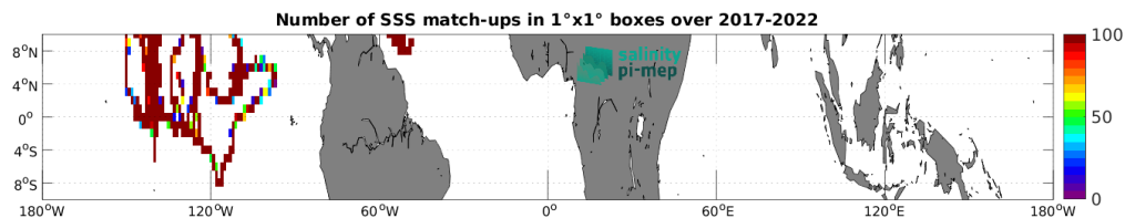
Figure 4: Number of SSS match-ups between Saildrone SSS and the SMAP SSS L3 v5.0 - 8-Day running (JPL) SSS product for the Equatorial Ocean 10N-10S Pi-MEP region over 1^\circ \times 1^\circ boxes and for the full satellite product period.
