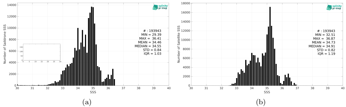
Figure 2: Histograms of SSS from Saildrone (a) and SMAP SSS L3 v5.0 - 8-Day running (JPL) (b) considering all match-up pairs per bins of 0.1 over the Equatorial Ocean 10N-10S Pi-MEP region and for the full satellite product period.
