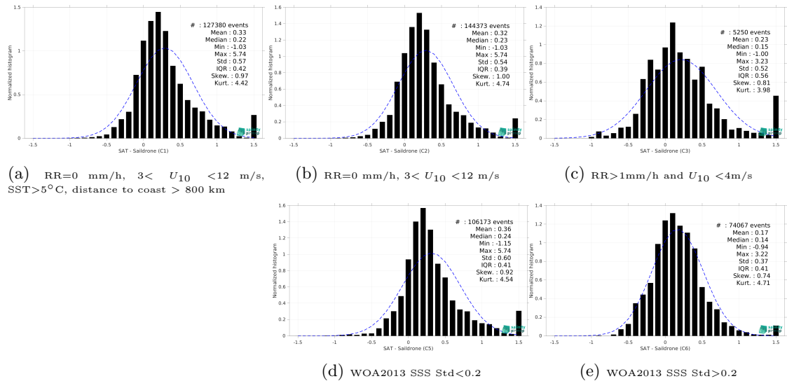
Figure 13: Normalized histogram of \Delta\text{SSS} (SMAP SSS L3 v5.0 - 8-Day running (JPL) - Saildrone) for 5 different subdatasets corresponding to: RR=0 mm/h, 3 < U_{10} < 12 m/s, SST >5^\circ\text{C} , distance to coast > 800 km (a), RR=0 mm/h, 3 < U_{10} < 12 m/s (b), RR >1 mm/h and U_{10} < 4 m/s (c), WOA2013 SSS Std <0.2 (d), WOA2013 SSS Std >0.2 (e).
