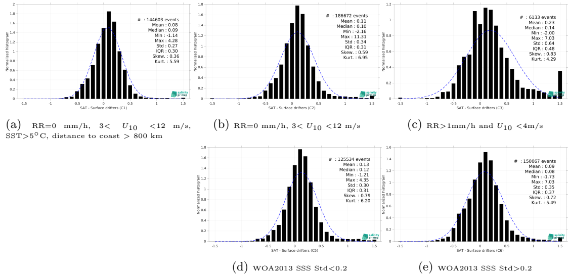
Figure 14: Normalized histogram of \Delta SSS (SMAP SSS L3 v5.0 - 8-Day running (JPL) - Surface drifters) for 5 different subdatasets corresponding to: RR=0 mm/h, 3 < U_{10} < 12 m/s, SST >5^\circ C, distance to coast > 800 km (a), RR=0 mm/h, 3 < U_{10} < 12 m/s (b), RR >1 mm/h and U_{10} < 4 m/s (c), WOA2013 SSS Std <0.2 (d), WOA2013 SSS Std >0.2 (e).
