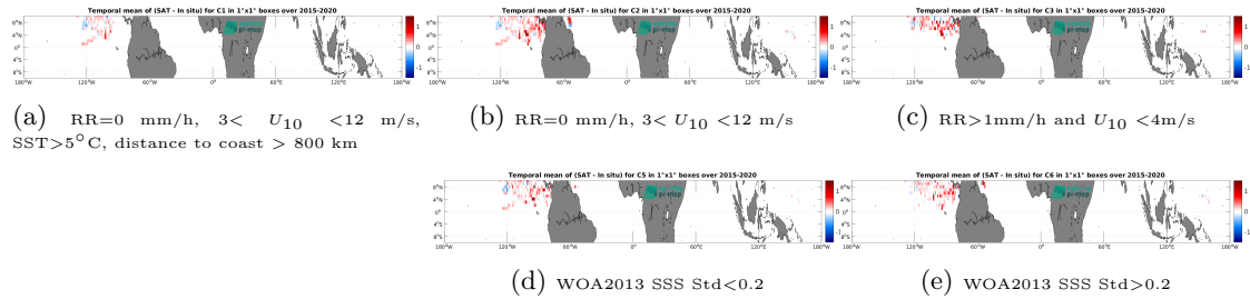
Figure 13: Temporal mean gridded over spatial boxes of size 1^\circ \times 1^\circ of \Delta SSS (SMAP SSS L3 v5.0 - 8-Day running (JPL) - Surface drifters) for 5 different subdatasets corresponding to: RR=0 mm/h, 3 < U_{10} < 12 m/s, SST >5^\circ C, distance to coast > 800 km (a), RR=0 mm/h, 3 < U_{10} < 12 m/s (b), RR >1 mm/h and U_{10} < 4 m/s (c), WOA2013 SSS Std <0.2 (d), WOA2013 SSS Std >0.2 (e).
