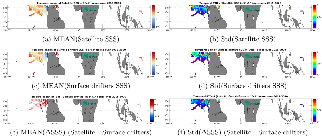
Figure 6: Temporal mean (left) and Std (right) of SSS from SMAP SSS L3 v5.0 - 8-Day running (JPL) (top), Surface drifters (middle), and of \Delta SSS (Satellite - Surface drifters). Only match-up pairs are used to generate these maps.
