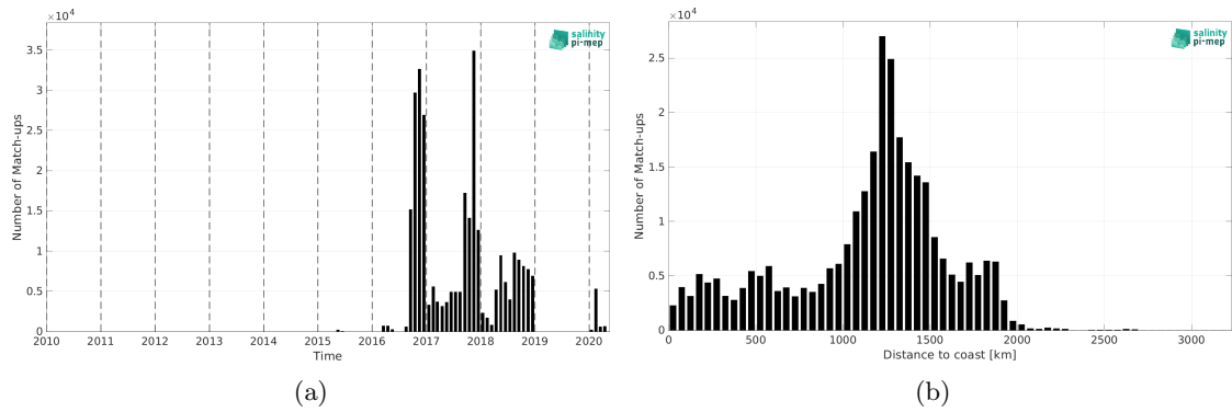
Figure 2: Number of match-ups between Surface drifters and SMAP SSS L3 v5.0 - 8-Day running (JPL) SSS as a function of time (a) and as function of the distance to coast (b) over the Equatorial Ocean 10N-10S Pi-MEP region and for the full satellite product period.
