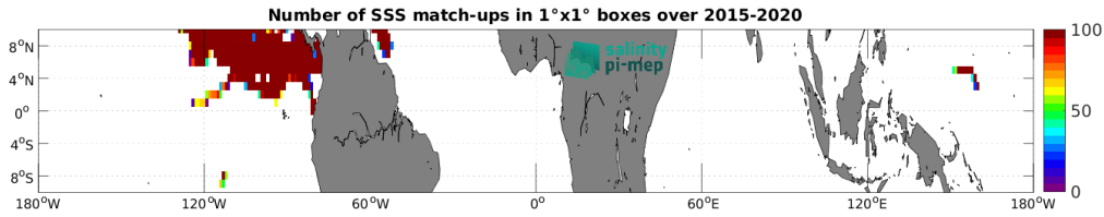
Figure 4: Number of SSS match-ups between Surface drifters SSS and the SMAP SSS L3 v5.0 - 8-Day running (JPL) SSS product for the Equatorial Ocean 10N-10S Pi-MEP region over 1^\circ \times 1^\circ boxes and for the full satellite product period.
