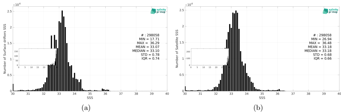
Figure 3: Histograms of SSS from Surface drifters (a) and SMAP SSS L3 v5.0 - 8-Day running (JPL) (b) considering all match-up pairs per bins of 0.1 over the Equatorial Ocean 10N-10S Pi-MEP region and for the full satellite product period.
