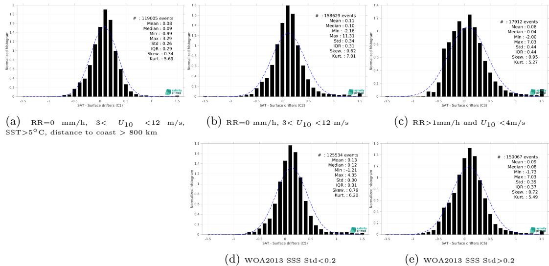
Figure 12: Normalized histogram of \Delta SSS (SMAP SSS L3 v5.0 - 8-Day running (JPL) - Surface drifters) for 5 different subdatasets corresponding to: RR=0 mm/h, 3 < U_{10} < 12 m/s, SST >5^\circ C, distance to coast > 800 km (a), RR=0 mm/h, 3 < U_{10} < 12 m/s (b), RR >1 mm/h and U_{10} < 4 m/s (c), WOA2013 SSS Std <0.2 (d), WOA2013 SSS Std >0.2 (e).
