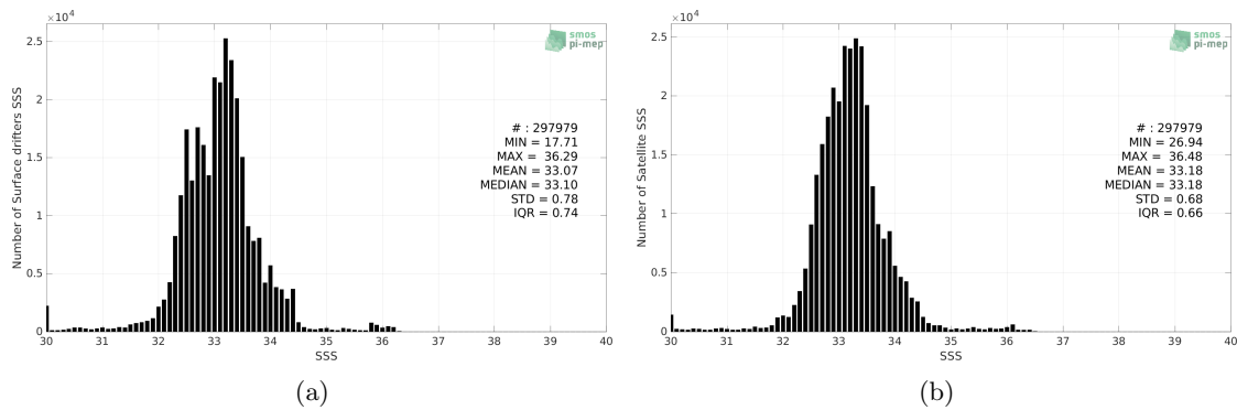
Figure 2: Histograms of SSS from Surface drifters (a) and SMAP SSS L3 v5.0 - 8-Day running (JPL) (b) considering all match-up pairs per bins of 0.1 over the Equatorial Ocean 10N-10S Pi-MEP region and for the full satellite product period.
