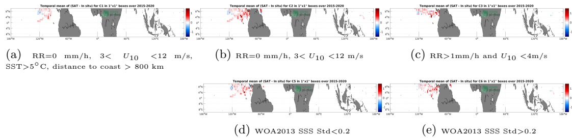
Figure 11: Temporal mean gridded over spatial boxes of size 1^\circ \times 1^\circ of \Delta SSS (SMAP SSS L3 v5.0 - 8-Day running (JPL) - Surface drifters) for 5 different subdatasets corresponding to: RR=0 mm/h, 3 < U_{10} < 12 m/s, SST>5°C, distance to coast > 800 km (a), RR=0 mm/h, 3 < U_{10} < 12 m/s (b), RR>1mm/h and U_{10} < 4 m/s (c), WOA2013 SSS Std<0.2 (d), WOA2013 SSS Std>0.2 (e).
