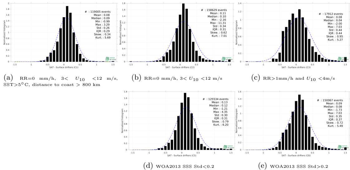
Figure 12: Normalized histogram of \Delta SSS (SMAP SSS L3 v5.0 - 8-Day running (JPL) - Surface drifters) for 5 different subdatasets corresponding to: RR=0 mm/h, 3 < U_{10} < 12 m/s, SST>5°C, distance to coast > 800 km (a), RR=0 mm/h, 3 < U_{10} < 12 m/s (b), RR>1mm/h and U_{10} < 4 m/s (c), WOA2013 SSS Std<0.2 (d), WOA2013 SSS Std>0.2 (e).
