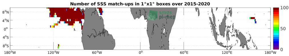
Figure 3: Number of SSS match-ups between Surface drifters SSS and the SMAP SSS L3 v5.0 - 8-Day running (JPL) SSS product for the Equatorial Ocean 10N-10S Pi-MEP region over 1^\circ \times 1^\circ boxes and for the full satellite product period.
