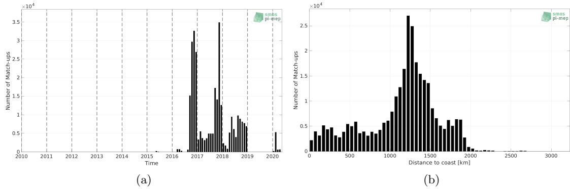
Figure 1: Number of match-ups between Surface drifters and SMAP SSS L3 v5.0 - 8-Day running (JPL) SSS as a function of time (a) and as function of the distance to coast (b) over the Equatorial Ocean 10N-10S Pi-MEP region and for the full satellite product period.
