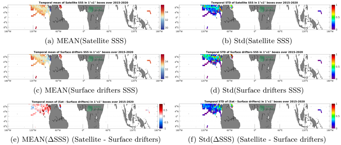
Figure 5: Temporal mean (left) and Std (right) of SSS from SMAP SSS L3 v5.0 - 8-Day running (JPL) (top), Surface drifters (middle), and of \Delta SSS (Satellite - Surface drifters). Only match-up pairs are used to generate these maps.
