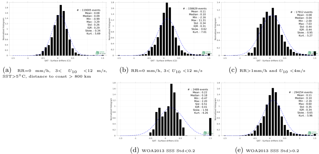
Figure 12: Normalized histogram of \Delta SSS (SMAP SSS L3 v5.0 - 8-Day running (JPL) - Surface drifters) for 5 different subdatasets corresponding to: RR=0 mm/h, 3 < U_{10} < 12 m/s, SST>5°C, distance to coast > 800 km (a), RR=0 mm/h, 3 < U_{10} < 12 m/s (b), RR>1mm/h and U_{10} < 4 m/s (c), WOA2013 SSS Std<0.2 (d), WOA2013 SSS Std>0.2 (e).
