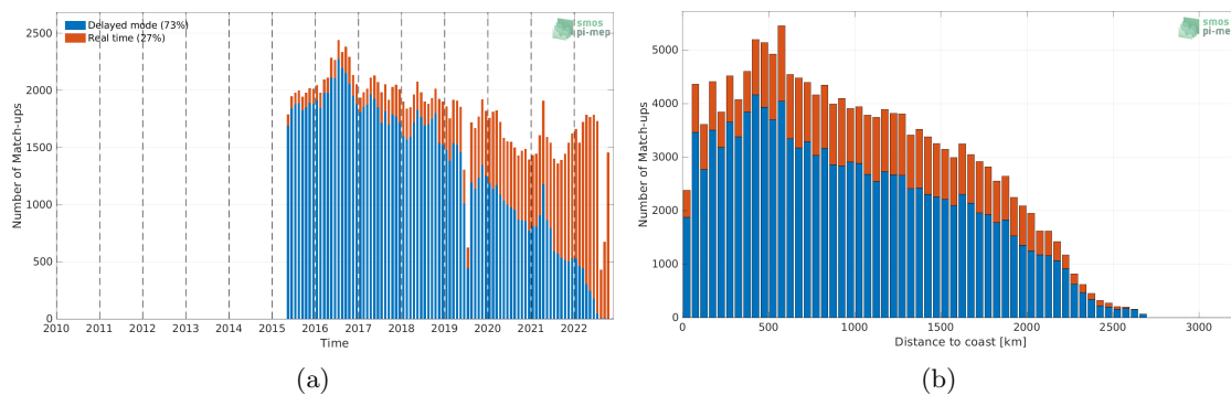
Figure 1: Number of match-ups between Argo and SMAP SSS L3 v5.0 - 8-Day running (JPL) SSS as a function of time (a) and as function of the distance to coast (b) over the Equatorial Ocean 10N-10S Pi-MEP region and for the full satellite product period.
