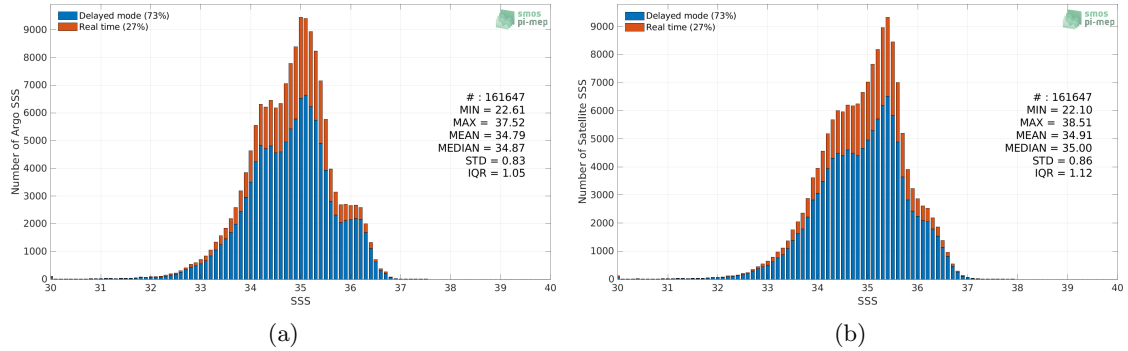
Figure 2: Histograms of SSS from Argo (a) and SMAP SSS L3 v5.0 - 8-Day running (JPL) (b) considering all match-up pairs per bins of 0.1 over the Equatorial Ocean 10N-10S Pi-MEP region and for the full satellite product period.
