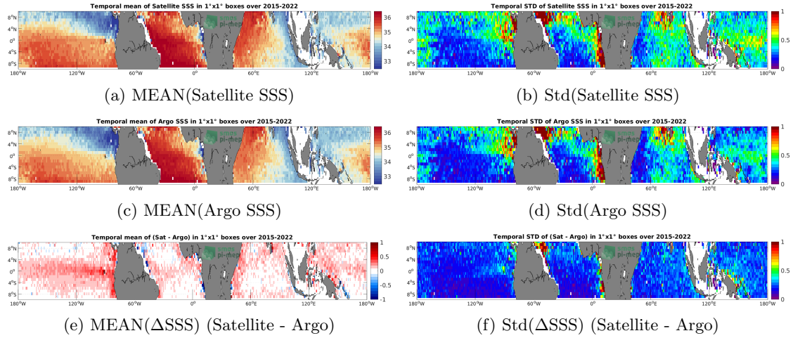
Figure 6: Temporal mean (left) and Std (right) of SSS from SMAP SSS L3 v5.0 - 8-Day running (JPL) (top), Argo (middle), and of \Delta SSS (Satellite - Argo). Only match-up pairs are used to generate these maps.
