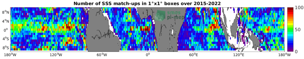
Figure 4: Number of SSS match-ups between Argo SSS and the SMAP SSS L3 v5.0 - 8-Day running (JPL) SSS product for the Equatorial Ocean 10N-10S Pi-MEP region over 1^\circ \times 1^\circ boxes and for the full satellite product period.
