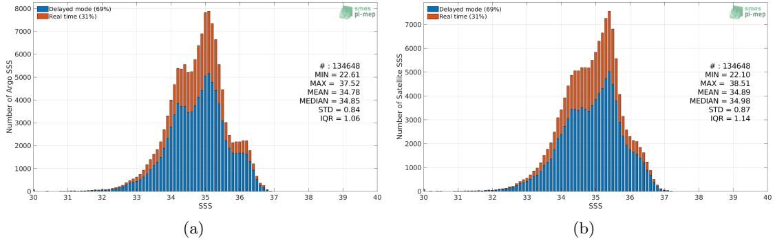
Figure 2: Histograms of SSS from Argo (a) and SMAP SSS L3 v5.0 - 8-Day running (JPL) (b) considering all match-up pairs per bins of 0.1 over the Equatorial Ocean 10N-10S Pi-MEP region and for the full satellite product period.
