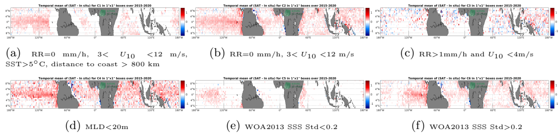
Figure 12: Temporal mean gridded over spatial boxes of size 1^\circ \times 1^\circ of \Delta SSS (SMAP SSS L3 v5.0 - 8-Day running (JPL) - Argo) for 6 different subdatasets corresponding to:RR=0 mm/h, 3 < U_{10} < 12 m/s, SST >5^\circ C, distance to coast > 800 km (a), RR=0 mm/h, 3 < U_{10} < 12 m/s (b), RR >1 mm/h and U_{10} < 4 m/s (c),MLD <20 m (d),WOA2013 SSS Std <0.2 (e),WOA2013 SSS Std >0.2 (f).
