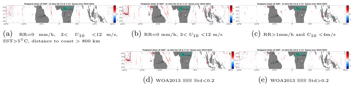
Figure 14: Temporal mean gridded over spatial boxes of size 1^\circ \times 1^\circ of \Delta SSS (SMAP SSS L3 v5.0 - Monthly (JPL) - TSG (SAMOS)) for 5 different subdatasets corresponding to: RR=0 mm/h, 3 < U_{10} < 12 m/s, SST>5°C, distance to coast > 800 km (a), RR=0 mm/h, 3 < U_{10} < 12 m/s (b), RR>1mm/h and U_{10} < 4 m/s (c), WOA2013 SSS Std<0.2 (d), WOA2013 SSS Std>0.2 (e).
