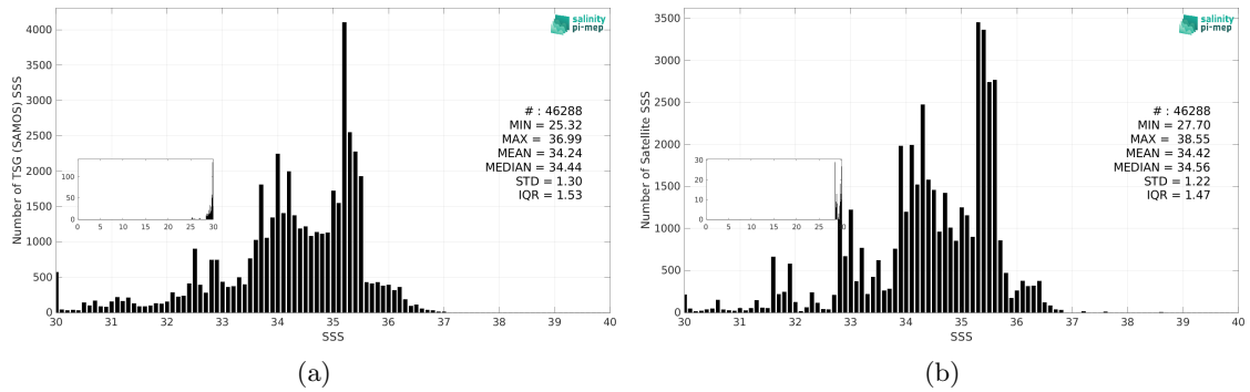
Figure 3: Histograms of SSS from TSG (SAMOS) (a) and SMAP SSS L3 v5.0 - Monthly (JPL) (b) considering all match-up pairs per bins of 0.1 over the Equatorial Ocean 10N-10S Pi-MEP region and for the full satellite product period.
