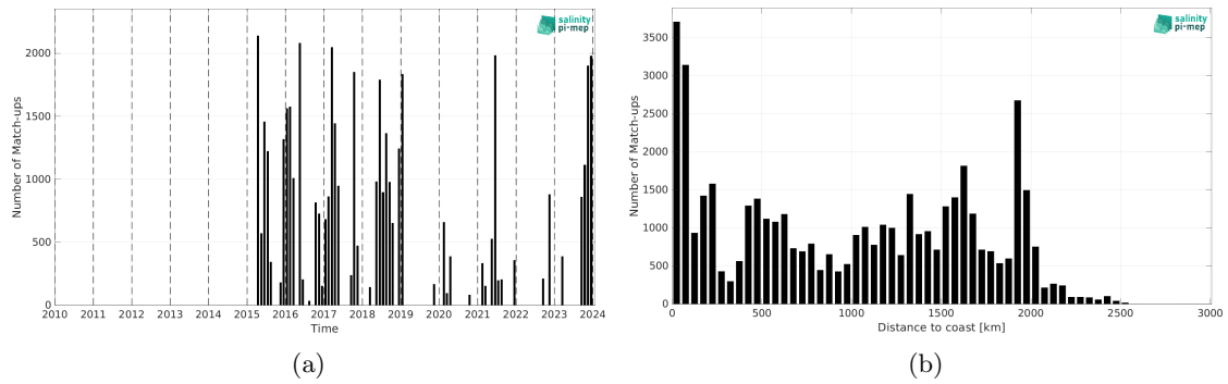
Figure 2: Number of match-ups between TSG (SAMOS) and SMAP SSS L3 v5.0 - Monthly (JPL) SSS as a function of time (a) and as function of the distance to coast (b) over the Equatorial Ocean 10N-10S Pi-MEP region and for the full satellite product period.
