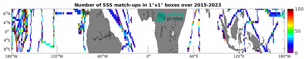
Figure 5: Number of SSS match-ups between TSG (SAMOS) SSS and the SMAP SSS L3 v5.0 - Monthly (JPL) SSS product for the Equatorial Ocean 10N-10S Pi-MEP region over 1^\circ \times 1^\circ boxes and for the full satellite product period.
