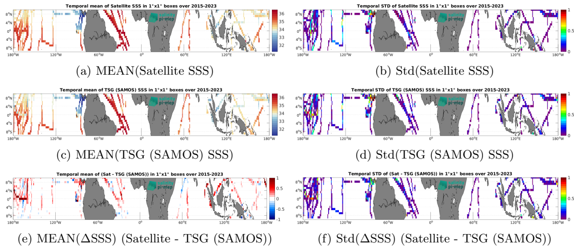
Figure 7: Temporal mean (left) and Std (right) of SSS from SMAP SSS L3 v5.0 - Monthly (JPL) (top), TSG (SAMOS) (middle), and of \Delta SSS (Satellite - TSG (SAMOS)). Only match-up pairs are used to generate these maps.
