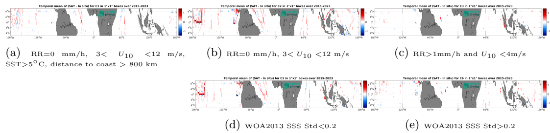
Figure 14: Temporal mean gridded over spatial boxes of size 1^\circ \times 1^\circ of \Delta\text{SSS} (SMAP SSS L3 v5.0 - Monthly (JPL) - TSG (SAMOS)) for 5 different subdatasets corresponding to:RR=0 mm/h, 3 < U_{10} < 12 m/s, SST>5°C, distance to coast > 800 km (a), RR=0 mm/h, 3 < U_{10} < 12 m/s (b), RR>1mm/h and U_{10} < 4 m/s (c), WOA2013 SSS Std<0.2 (d), WOA2013 SSS Std>0.2 (e).
