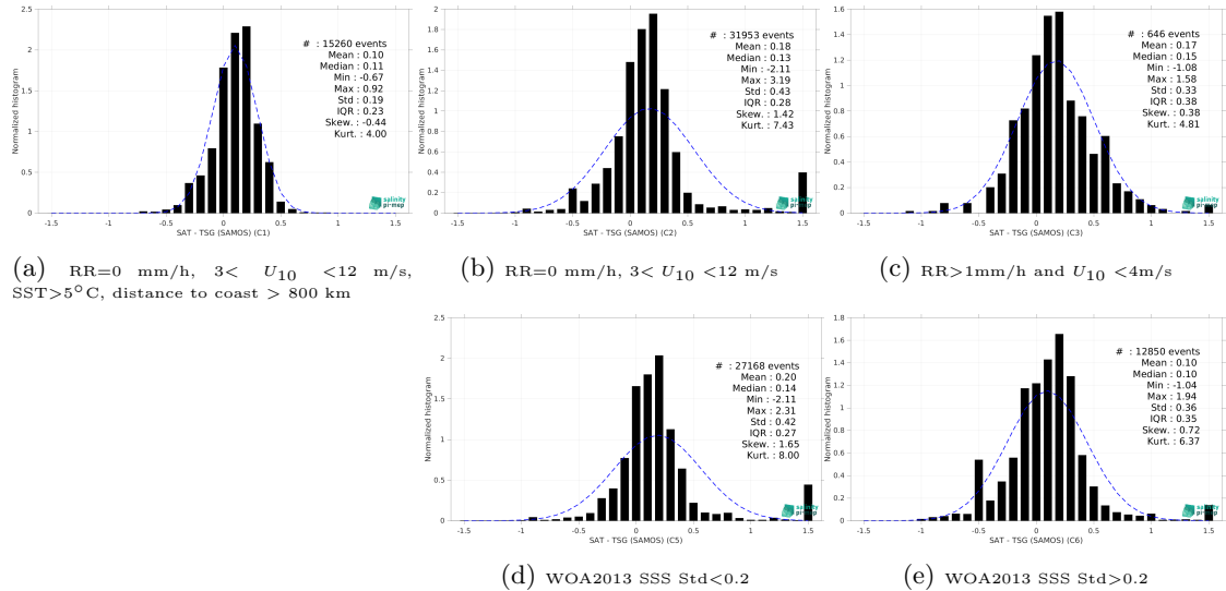
Figure 15: Normalized histogram of \Delta\text{SSS} (SMAP SSS L3 v5.0 - Monthly (JPL) - TSG (SAMOS)) for 5 different subdatasets corresponding to: RR=0 mm/h, 3 < U_{10} < 12 m/s, SST>5°C, distance to coast > 800 km (a), RR=0 mm/h, 3 < U_{10} < 12 m/s (b), RR>1mm/h and U_{10} < 4 m/s (c), WOA2013 SSS Std<0.2 (d), WOA2013 SSS Std>0.2 (e).
