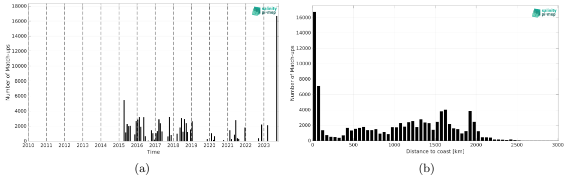
Figure 1: Number of match-ups between TSG (SAMOS) and SMAP SSS L3 v5.0 - Monthly (JPL) SSS as a function of time (a) and as function of the distance to coast (b) over the Equatorial Ocean 10N-10S Pi-MEP region and for the full satellite product period.
