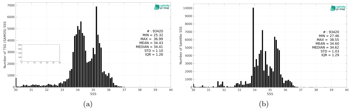
Figure 2: Histograms of SSS from TSG (SAMOS) (a) and SMAP SSS L3 v5.0 - Monthly (JPL) (b) considering all match-up pairs per bins of 0.1 over the Equatorial Ocean 10N-10S Pi-MEP region and for the full satellite product period.
