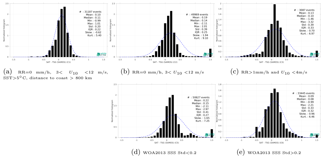
Figure 13: Normalized histogram of \Delta SSS (SMAP SSS L3 v5.0 - Monthly (JPL) - TSG (SAMOS)) for 5 different subdatasets corresponding to: RR=0 mm/h, 3 < U_{10} < 12 m/s, SST >5^\circ\text{C} , distance to coast > 800 km (a), RR=0 mm/h, 3 < U_{10} < 12 m/s (b), RR >1 mm/h and U_{10} < 4 m/s (c), WOA2013 SSS Std <0.2 (d), WOA2013 SSS Std >0.2 (e).
