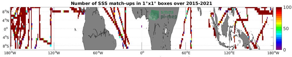
Figure 4: Number of SSS match-ups between TSG (SAMOS) SSS and the SMAP SSS L3 v5.0 - Monthly (JPL) SSS product for the Equatorial Ocean 10N-10S Pi-MEP region over 1^\circ \times 1^\circ boxes and for the full satellite product period.
