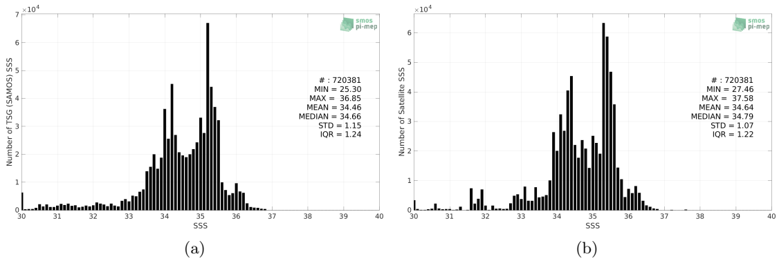
Figure 2: Histograms of SSS from TSG (SAMOS) (a) and SMAP SSS L3 v5.0 - Monthly (JPL) (b) considering all match-up pairs per bins of 0.1 over the Equatorial Ocean 10N-10S Pi-MEP region and for the full satellite product period.
