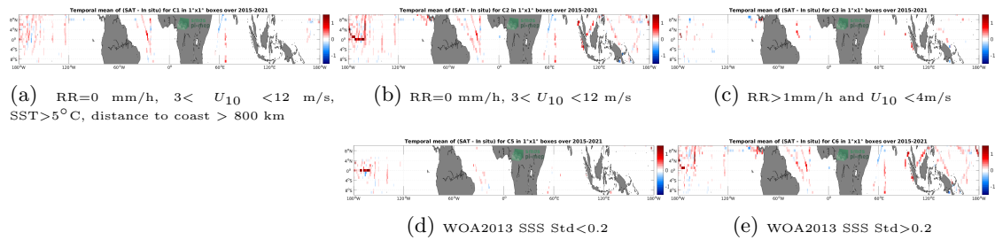
Figure 12: Temporal mean gridded over spatial boxes of size 1^\circ \times 1^\circ of \Delta SSS (SMAP SSS L3 v5.0 - Monthly (JPL) - TSG (SAMOS)) for 5 different subdatasets corresponding to:RR=0 mm/h, 3 < U_{10} < 12 m/s, SST>5°C, distance to coast > 800 km (a), RR=0 mm/h, 3 < U_{10} < 12 m/s (b), RR>1mm/h and U_{10} < 4 m/s (c), WOA2013 SSS Std<0.2 (d), WOA2013 SSS Std>0.2 (e).
