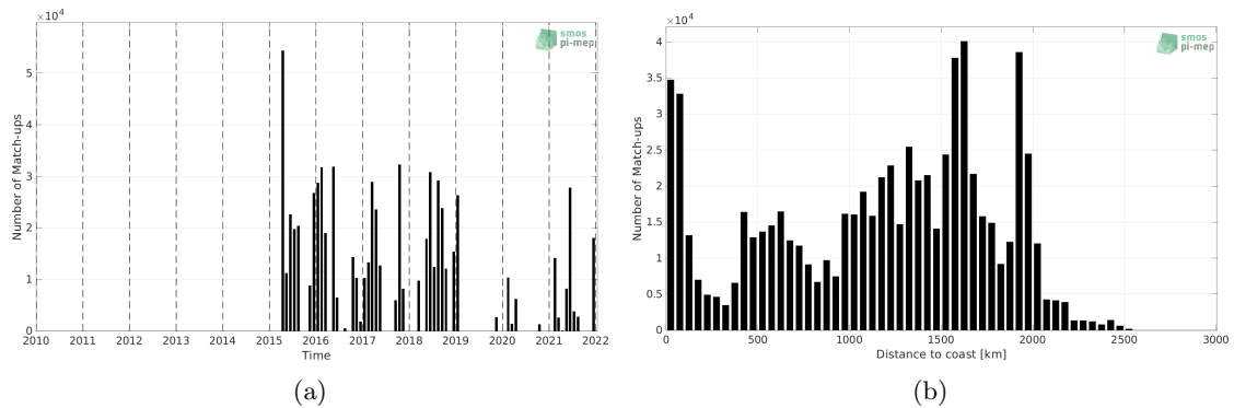
Figure 1: Number of match-ups between TSG (SAMOS) and SMAP SSS L3 v5.0 - Monthly (JPL) SSS as a function of time (a) and as function of the distance to coast (b) over the Equatorial Ocean 10N-10S Pi-MEP region and for the full satellite product period.
