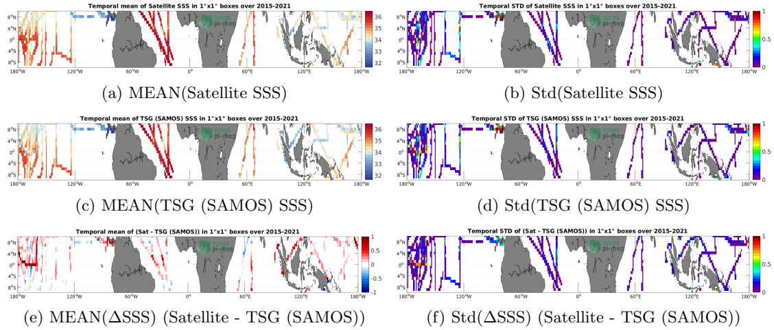
Figure 6: Temporal mean (left) and Std (right) of SSS from SMAP SSS L3 v5.0 - Monthly (JPL) (top), TSG (SAMOS) (middle), and of \Delta SSS (Satellite - TSG (SAMOS)). Only match-up pairs are used to generate these maps.
