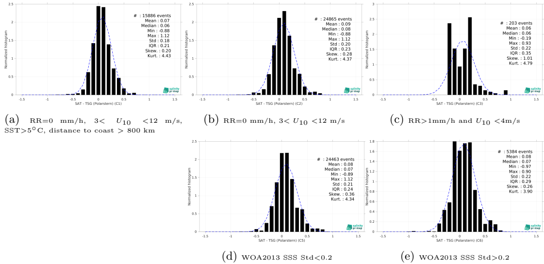
Figure 15: Normalized histogram of \Delta\text{SSS} (SMAP SSS L3 v5.0 - Monthly (JPL) - TSG (Polarstern)) for 5 different subdatasets corresponding to: RR=0 mm/h, 3 < U_{10} < 12 m/s, SST>5°C, distance to coast > 800 km (a), RR=0 mm/h, 3 < U_{10} < 12 m/s (b), RR>1mm/h and U_{10} < 4 m/s (c), WOA2013 SSS Std<0.2 (d), WOA2013 SSS Std>0.2 (e).
