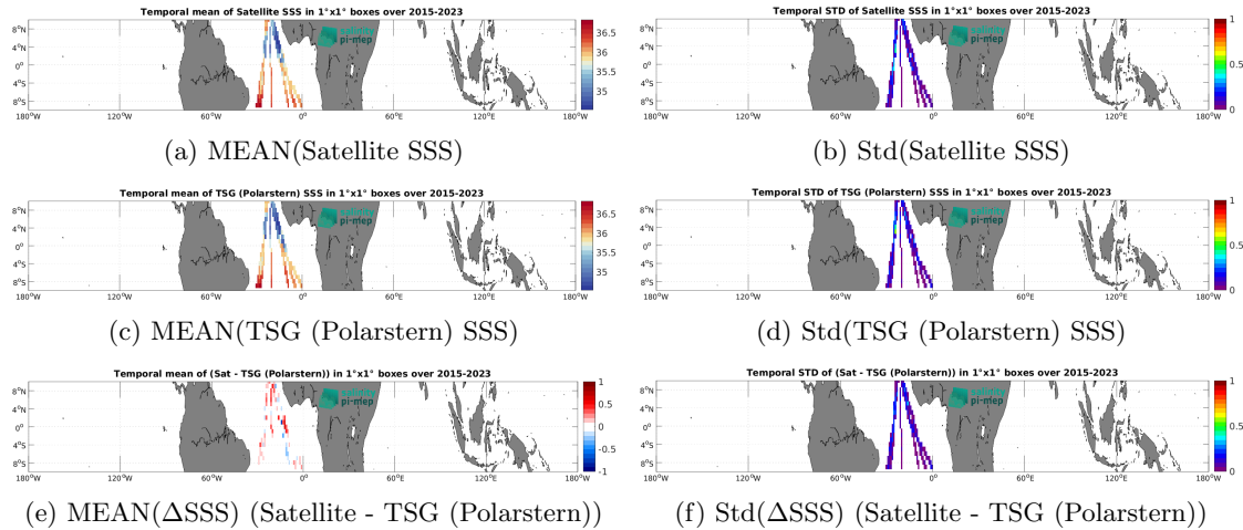
Figure 7: Temporal mean (left) and Std (right) of SSS from SMAP SSS L3 v5.0 - Monthly (JPL) (top), TSG (Polarstern) (middle), and of \Delta SSS (Satellite - TSG (Polarstern)). Only match-up pairs are used to generate these maps.
