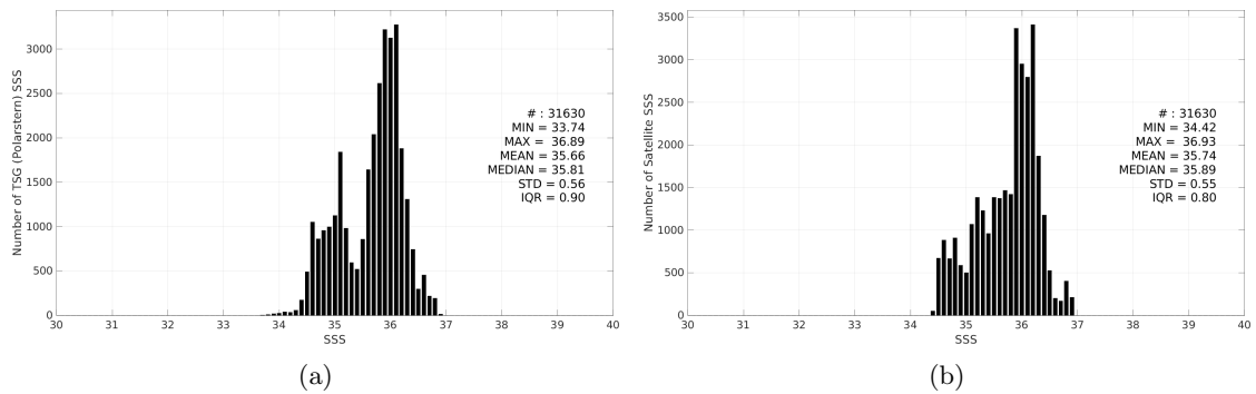
Figure 3: Histograms of SSS from TSG (Polarstern) (a) and SMAP SSS L3 v5.0 - Monthly (JPL) (b) considering all match-up pairs per bins of 0.1 over the Equatorial Ocean 10N-10S Pi-MEP region and for the full satellite product period.
