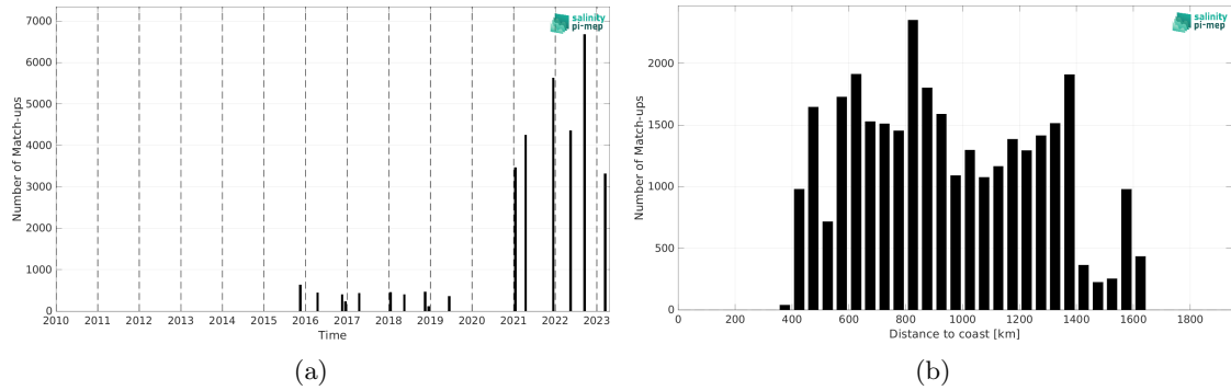
Figure 2: Number of match-ups between TSG (Polarstern) and SMAP SSS L3 v5.0 - Monthly (JPL) SSS as a function of time (a) and as function of the distance to coast (b) over the Equatorial Ocean 10N-10S Pi-MEP region and for the full satellite product period.
