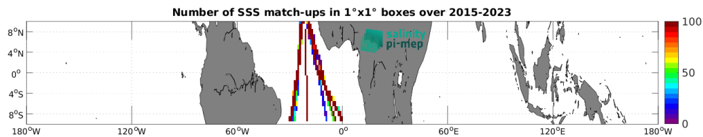
Figure 5: Number of SSS match-ups between TSG (Polarstern) SSS and the SMAP SSS L3 v5.0 - Monthly (JPL) SSS product for the Equatorial Ocean 10N-10S Pi-MEP region over 1^\circ \times 1^\circ boxes and for the full satellite product period.
