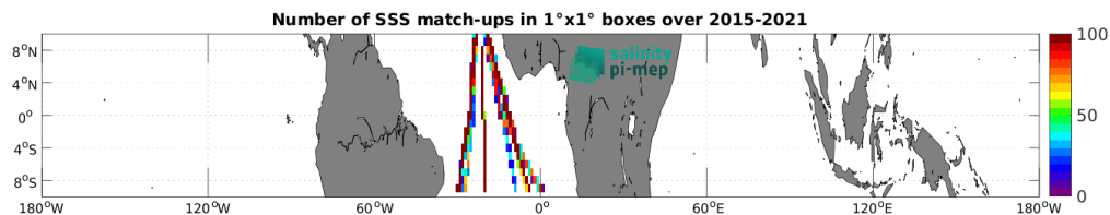
Figure 4: Number of SSS match-ups between TSG (Polarstern) SSS and the SMAP SSS L3 v5.0 - Monthly (JPL) SSS product for the Equatorial Ocean 10N-10S Pi-MEP region over 1^\circ \times 1^\circ boxes and for the full satellite product period.
