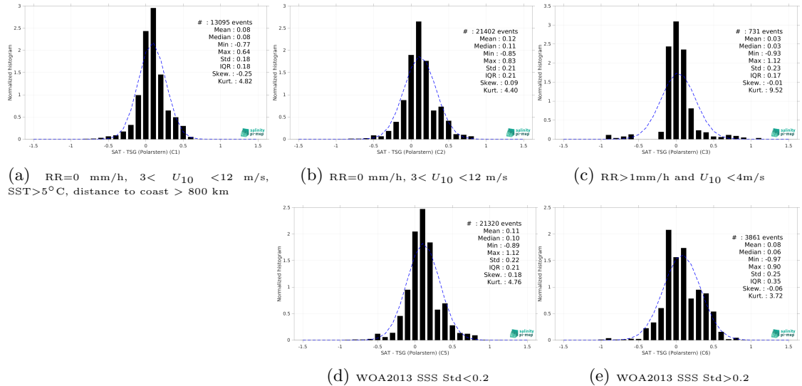
Figure 13: Normalized histogram of \Delta SSS (SMAP SSS L3 v5.0 - Monthly (JPL) - TSG (Polarstern)) for 5 different subdatasets corresponding to: RR=0 mm/h, 3 < U_{10} < 12 m/s, SST >5^\circ C, distance to coast > 800 km (a), RR=0 mm/h, 3 < U_{10} < 12 m/s (b), RR >1 mm/h and U_{10} < 4 m/s (c), WOA2013 SSS Std <0.2 (d), WOA2013 SSS Std >0.2 (e).
