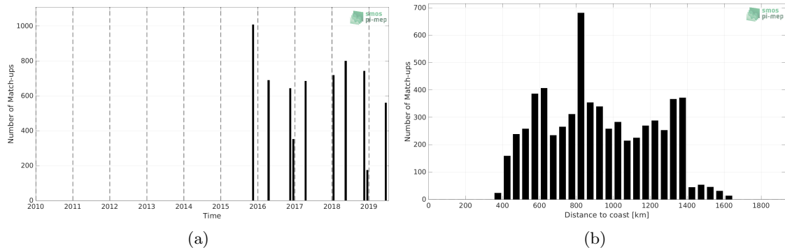
Figure 1: Number of match-ups between TSG (Polarstern) and SMAP SSS L3 v5.0 - Monthly (JPL) SSS as a function of time (a) and as function of the distance to coast (b) over the Equatorial Ocean 10N-10S Pi-MEP region and for the full satellite product period.
