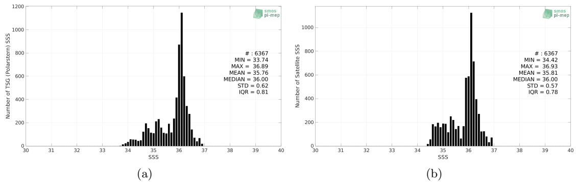
Figure 2: Histograms of SSS from TSG (Polarstern) (a) and SMAP SSS L3 v5.0 - Monthly (JPL) (b) considering all match-up pairs per bins of 0.1 over the Equatorial Ocean 10N-10S Pi-MEP region and for the full satellite product period.
