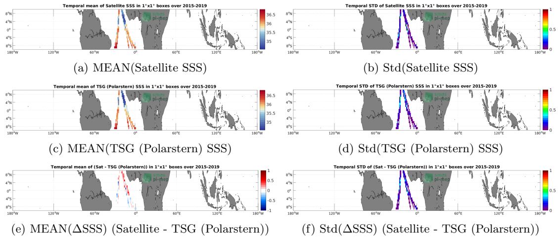
Figure 6: Temporal mean (left) and Std (right) of SSS from SMAP SSS L3 v5.0 - Monthly (JPL) (top), TSG (Polarstern) (middle), and of \Delta SSS (Satellite - TSG (Polarstern)). Only match-up pairs are used to generate these maps.
