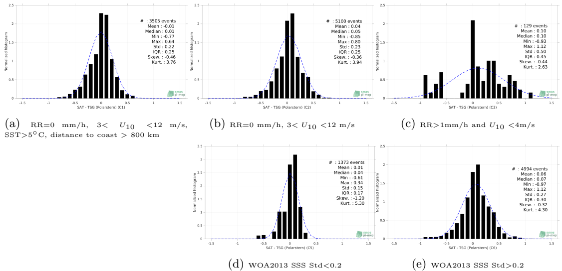
Figure 13: Normalized histogram of \Delta SSS (SMAP SSS L3 v5.0 - Monthly (JPL) - TSG (Polarstern)) for 5 different subdatasets corresponding to: RR=0 mm/h, 3 < U_{10} < 12 m/s, SST >5^\circ\text{C} , distance to coast > 800 km (a), RR=0 mm/h, 3 < U_{10} < 12 m/s (b), RR >1 mm/h and U_{10} < 4 m/s (c), WOA2013 SSS Std <0.2 (d), WOA2013 SSS Std >0.2 (e).
