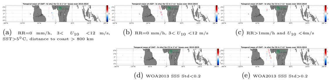
Figure 12: Temporal mean gridded over spatial boxes of size 1°x1° of ΔSSS (SMAP SSS L3 v5.0 - Monthly (JPL) - TSG (Polarstern)) for 5 different subdatasets corresponding to:RR=0 mm/h, 3 < U 10 < 12 m/s, SST>5°C, distance to coast > 800 km (a), RR=0 mm/h, 3 < U 10 < 12 m/s (b), RR>1mm/h and U 10 < 4m/s (c), WOA2013 SSS Std<0.2 (d), WOA2013 SSS Std>0.2 (e).
