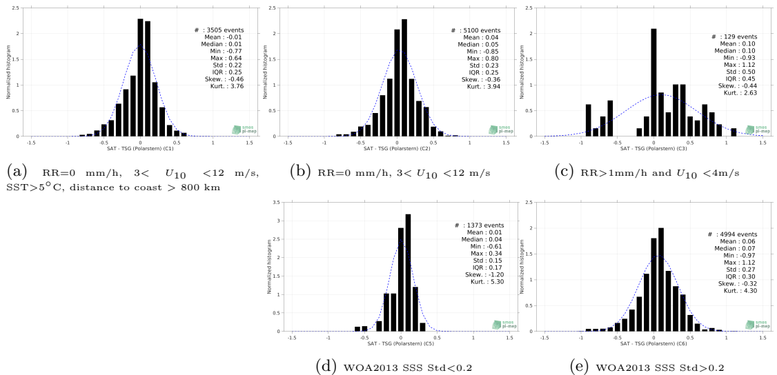
Figure 13: Normalized histogram of ΔSSS (SMAP SSS L3 v5.0 - Monthly (JPL) - TSG (Polarstern)) for 5 different subdatasets corresponding to: RR=0 mm/h, 3 < U 10 < 12 m/s, SST>5°C, distance to coast > 800 km (a), RR=0 mm/h, 3 < U 10 < 12 m/s (b), RR>1mm/h and U 10 < 4m/s (c), WOA2013 SSS Std<0.2 (d), WOA2013 SSS Std>0.2 (e).
