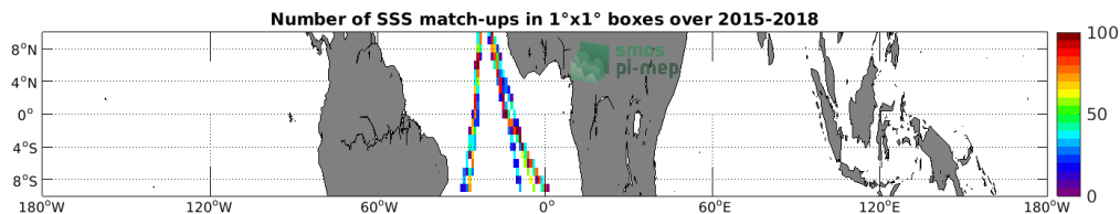
Figure 4: Number of SSS match-ups between TSG (Polarstern) SSS and the SMAP SSS L3 v5.0 - Monthly (JPL) SSS product for the Equatorial Ocean 10N-10S Pi-MEP region over 1°x1° boxes and for the full satellite product period.
