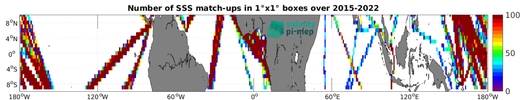
Figure 5: Number of SSS match-ups between TSG (LEGOS-DM) SSS and the SMAP SSS L3 v5.0 - Monthly (JPL) SSS product for the Equatorial Ocean 10N-10S Pi-MEP region over 1°×1° boxes and for the full satellite product period.
