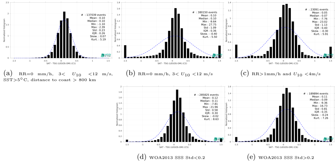
Figure 13: Normalized histogram of \Delta SSS (SMAP SSS L3 v5.0 - Monthly (JPL) - TSG (LEGOS-DM)) for 5 different subdatasets corresponding to: RR=0 mm/h, 3 < U_{10} < 12 m/s, SST >5^\circ\text{C} , distance to coast > 800 km (a), RR=0 mm/h, 3 < U_{10} < 12 m/s (b), RR >1 mm/h and U_{10} < 4 m/s (c), WOA2013 SSS Std <0.2 (d), WOA2013 SSS Std >0.2 (e).
