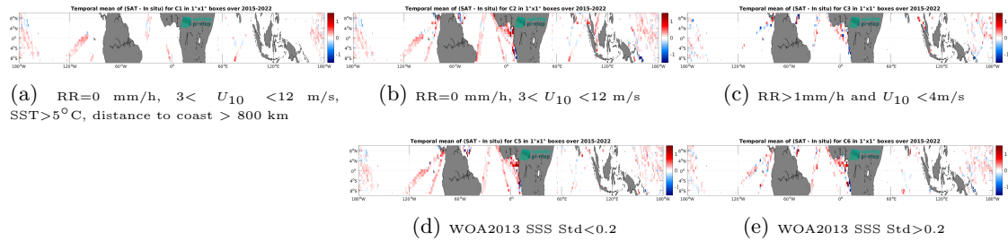
Figure 12: Temporal mean gridded over spatial boxes of size 1^\circ \times 1^\circ of \Delta SSS (SMAP SSS L3 v5.0 - Monthly (JPL) - TSG (LEGOS-DM)) for 5 different subdatasets corresponding to:RR=0 mm/h, 3 < U_{10} < 12 m/s, SST >5^\circ\text{C} , distance to coast > 800 km (a), RR=0 mm/h, 3 < U_{10} < 12 m/s (b), RR >1 mm/h and U_{10} < 4 m/s (c), WOA2013 SSS Std <0.2 (d), WOA2013 SSS Std >0.2 (e).
