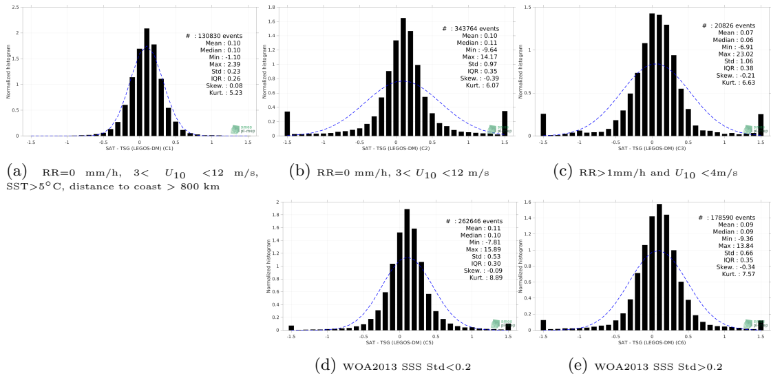
Figure 13: Normalized histogram of \Delta SSS (SMAP SSS L3 v5.0 - Monthly (JPL) - TSG (LEGOS-DM)) for 5 different subdatasets corresponding to: RR=0 mm/h, 3 < U_{10} < 12 m/s, SST >5^\circ C, distance to coast > 800 km (a), RR=0 mm/h, 3 < U_{10} < 12 m/s (b), RR >1 mm/h and U_{10} < 4 m/s (c), WOA2013 SSS Std <0.2 (d), WOA2013 SSS Std >0.2 (e).
