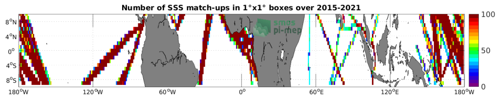
Figure 4: Number of SSS match-ups between TSG (LEGOS-DM) SSS and the SMAP SSS L3 v5.0 - Monthly (JPL) SSS product for the Equatorial Ocean 10N-10S Pi-MEP region over 1^\circ \times 1^\circ boxes and for the full satellite product period.
