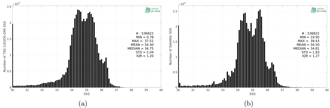
Figure 2: Histograms of SSS from TSG (LEGOS-DM) (a) and SMAP SSS L3 v5.0 - Monthly (JPL) (b) considering all match-up pairs per bins of 0.1 over the Equatorial Ocean 10N-10S Pi-MEP region and for the full satellite product period.
