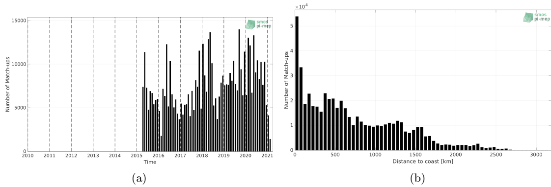
Figure 1: Number of match-ups between TSG (LEGOS-DM) and SMAP SSS L3 v5.0 - Monthly (JPL) SSS as a function of time (a) and as function of the distance to coast (b) over the Equatorial Ocean 10N-10S Pi-MEP region and for the full satellite product period.
