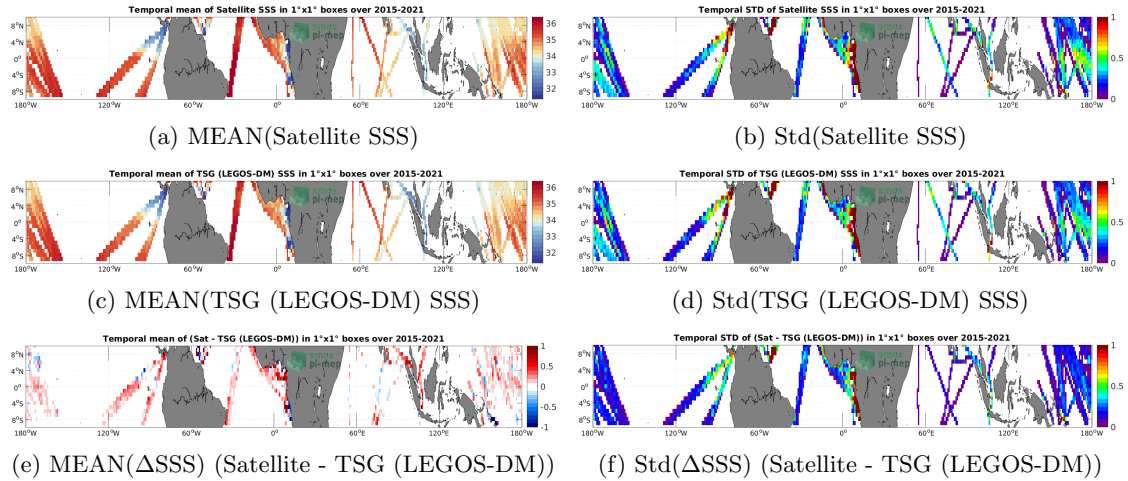
Figure 6: Temporal mean (left) and Std (right) of SSS from SMAP SSS L3 v5.0 - Monthly (JPL) (top), TSG (LEGOS-DM) (middle), and of \Delta SSS (Satellite - TSG (LEGOS-DM)). Only match-up pairs are used to generate these maps.
