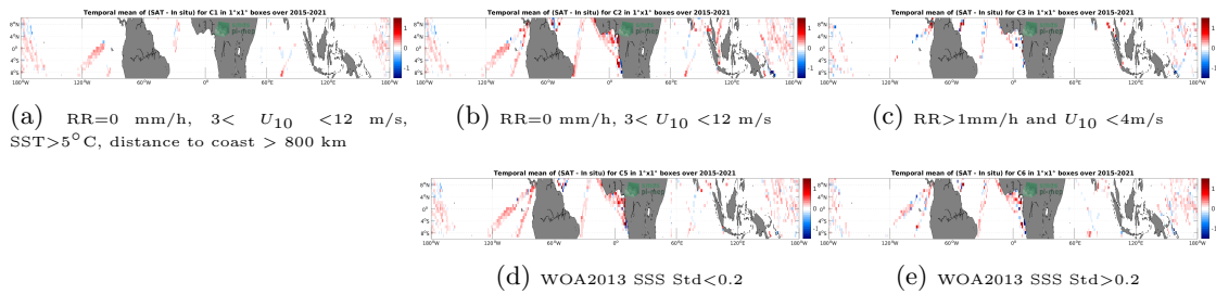
Figure 12: Temporal mean gridded over spatial boxes of size 1^\circ \times 1^\circ of \Delta SSS (SMAP SSS L3 v5.0 - Monthly (JPL) - TSG (LEGOS-DM)) for 5 different subdatasets corresponding to: RR=0 mm/h, 3 < U_{10} < 12 m/s, SST >5^\circ C, distance to coast > 800 km (a), RR=0 mm/h, 3 < U_{10} < 12 m/s (b), RR >1 mm/h and U_{10} < 4 m/s (c), WOA2013 SSS Std <0.2 (d), WOA2013 SSS Std >0.2 (e).
