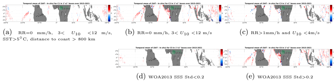
Figure 12: Temporal mean gridded over spatial boxes of size 1^\circ \times 1^\circ of \Delta SSS (SMAP SSS L3 v5.0 - Monthly (JPL) - TSG (LEGOS-DM)) for 5 different subdatasets corresponding to:RR=0 mm/h, 3 < U_{10} < 12 m/s, SST > 5^\circ C , distance to coast > 800 km (a), RR=0 mm/h, 3 < U_{10} < 12 m/s (b), RR>1mm/h and U_{10} < 4 m/s (c), WOA2013 SSS Std<0.2 (d), WOA2013 SSS Std>0.2 (e).
