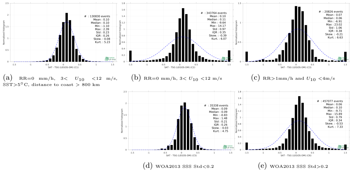
Figure 13: Normalized histogram of \Delta SSS (SMAP SSS L3 v5.0 - Monthly (JPL) - TSG (LEGOS-DM)) for 5 different subdatasets corresponding to: RR=0 mm/h, 3 < U_{10} < 12 m/s, SST > 5^\circ C , distance to coast > 800 km (a), RR=0 mm/h, 3 < U_{10} < 12 m/s (b), RR>1mm/h and U_{10} < 4 m/s (c), WOA2013 SSS Std<0.2 (d), WOA2013 SSS Std>0.2 (e).
