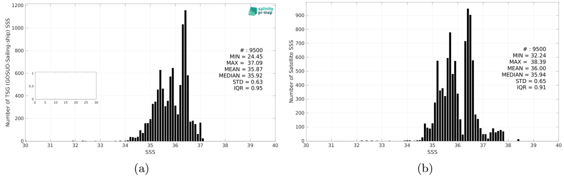
Figure 3: Histograms of SSS from TSG (GOSUD-Sailing-ship) (a) and SMAP SSS L3 v5.0 - Monthly (JPL) (b) considering all match-up pairs per bins of 0.1 over the Equatorial Ocean 10N-10S Pi-MEP region and for the full satellite product period.
