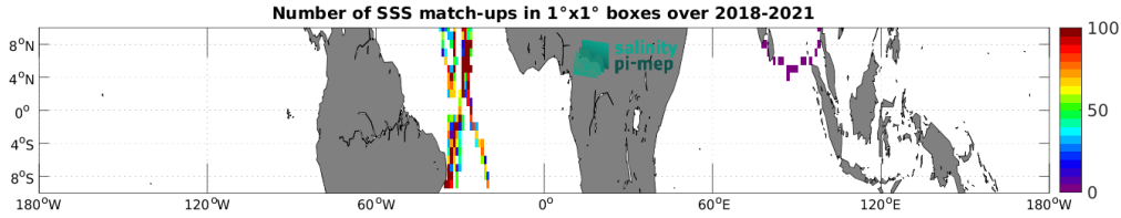
Figure 5: Number of SSS match-ups between TSG (GOSUD-Sailing-ship) SSS and the SMAP SSS L3 v5.0 - Monthly (JPL) SSS product for the Equatorial Ocean 10N-10S Pi-MEP region over 1^\circ \times 1^\circ boxes and for the full satellite product period.
