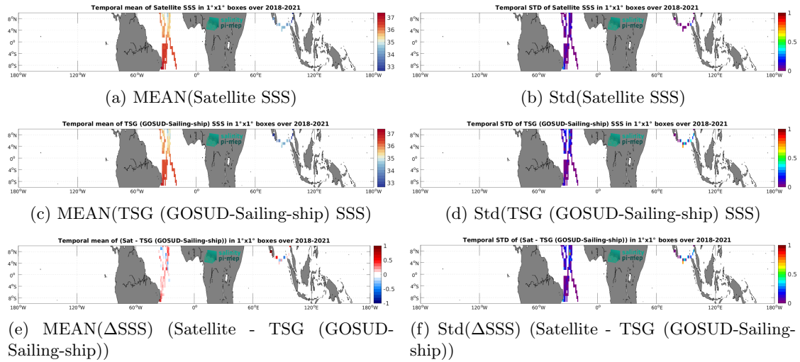
Figure 7: Temporal mean (left) and Std (right) of SSS from SMAP SSS L3 v5.0 - Monthly (JPL) (top), TSG (GOSUD-Sailing-ship) (middle), and of \Delta SSS (Satellite - TSG (GOSUD-Sailing-ship)). Only match-up pairs are used to generate these maps.
