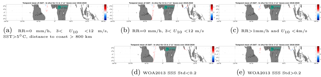
Figure 12: Temporal mean gridded over spatial boxes of size 1^\circ \times 1^\circ of \Delta SSS (SMAP SSS L3 v5.0 - Monthly (JPL) - TSG (GOSUD-Sailing-ship)) for 5 different subdatasets corresponding to: RR=0 mm/h, 3 < U_{10} < 12 m/s, SST>5°C, distance to coast > 800 km (a), RR=0 mm/h, 3 < U_{10} < 12 m/s (b), RR>1mm/h and U_{10} < 4 m/s (c), WOA2013 SSS Std<0.2 (d), WOA2013 SSS Std>0.2 (e).
