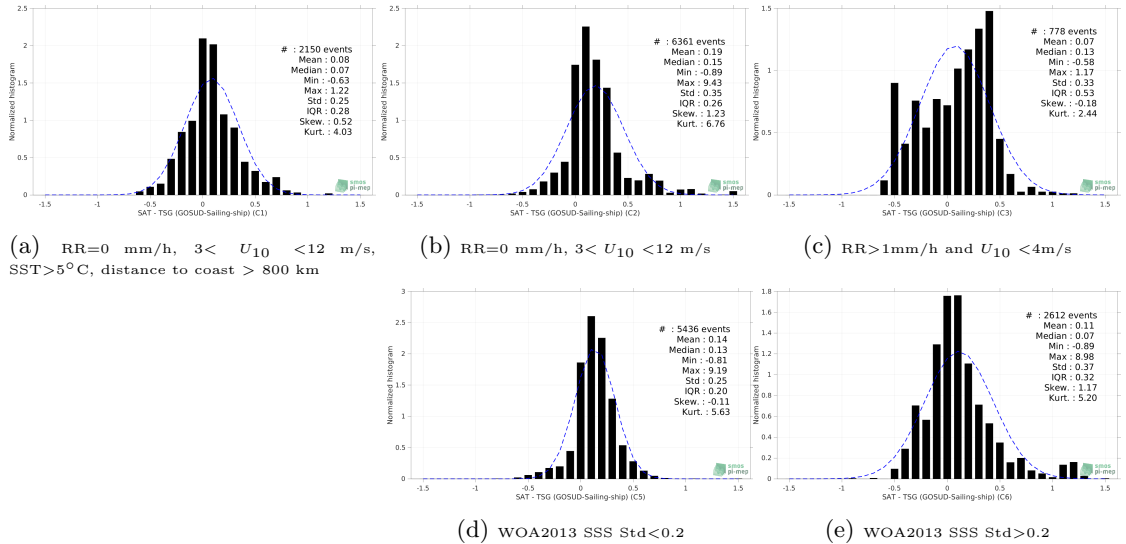
Figure 13: Normalized histogram of \Delta SSS (SMAP SSS L3 v5.0 - Monthly (JPL) - TSG (GOSUD-Sailing-ship)) for 5 different subdatasets corresponding to: RR=0 mm/h, 3 < U_{10} < 12 m/s, SST>5°C, distance to coast > 800 km (a), RR=0 mm/h, 3 < U_{10} < 12 m/s (b), RR>1mm/h and U_{10} < 4 m/s (c), WOA2013 SSS Std<0.2 (d), WOA2013 SSS Std>0.2 (e).
