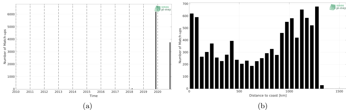
Figure 1: Number of match-ups between TSG (GOSUD-Sailing-ship) and SMAP SSS L3 v5.0 - Monthly (JPL) SSS as a function of time (a) and as function of the distance to coast (b) over the Equatorial Ocean 10N-10S Pi-MEP region and for the full satellite product period.
