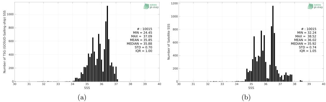
Figure 2: Histograms of SSS from TSG (GOSUD-Sailing-ship) (a) and SMAP SSS L3 v5.0 - Monthly (JPL) (b) considering all match-up pairs per bins of 0.1 over the Equatorial Ocean 10N-10S Pi-MEP region and for the full satellite product period.
