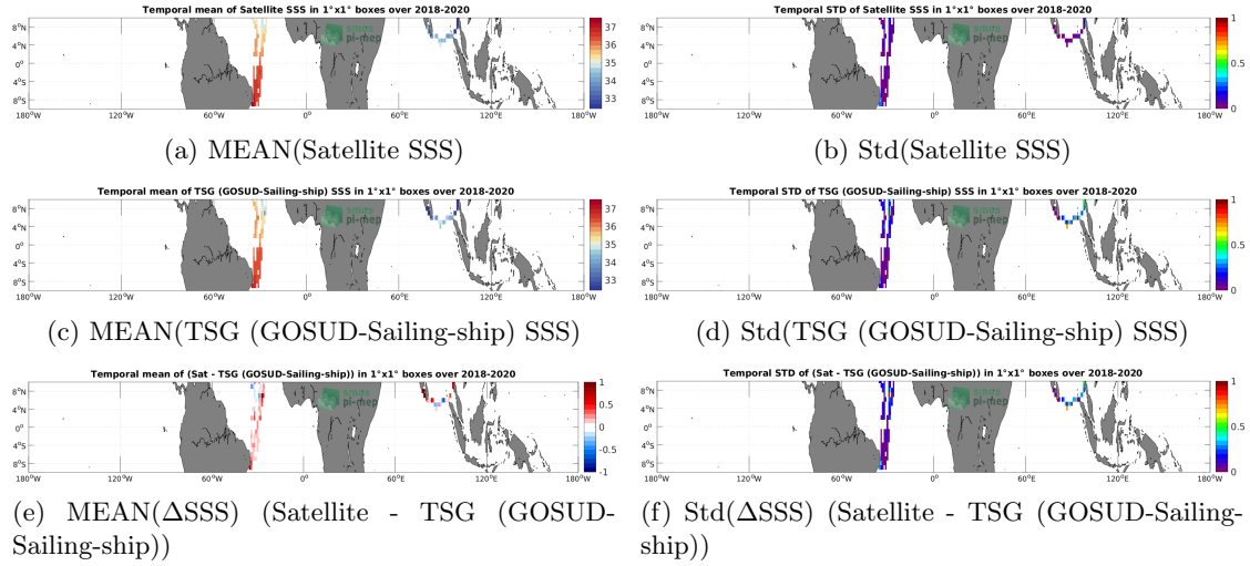
Figure 6: Temporal mean (left) and Std (right) of SSS from SMAP SSS L3 v5.0 - Monthly (JPL) (top), TSG (GOSUD-Sailing-ship) (middle), and of \Delta SSS (Satellite - TSG (GOSUD-Sailing-ship)). Only match-up pairs are used to generate these maps.
