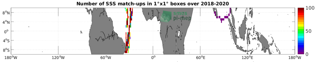
Figure 4: Number of SSS match-ups between TSG (GOSUD-Sailing-ship) SSS and the SMAP SSS L3 v5.0 - Monthly (JPL) SSS product for the Equatorial Ocean 10N-10S Pi-MEP region over 1^\circ \times 1^\circ boxes and for the full satellite product period.
