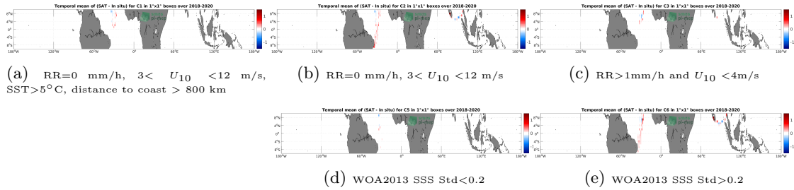
Figure 12: Temporal mean gridded over spatial boxes of size 1^\circ \times 1^\circ of \Delta SSS (SMAP SSS L3 v5.0 - Monthly (JPL) - TSG (GOSUD-Sailing-ship)) for 5 different subdatasets corresponding to: RR=0 mm/h, 3 < U_{10} < 12 m/s, SST>5°C, distance to coast > 800 km (a), RR=0 mm/h, 3 < U_{10} < 12 m/s (b), RR>1mm/h and U_{10} < 4 m/s (c), WOA2013 SSS Std<0.2 (d), WOA2013 SSS Std>0.2 (e).
