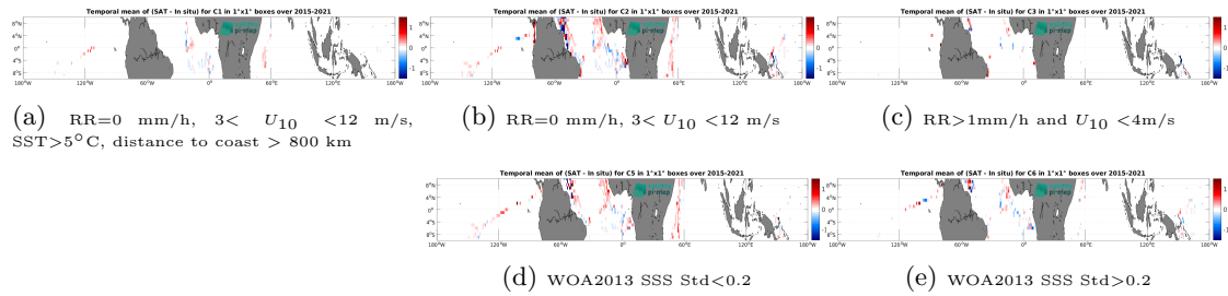
Figure 14: Temporal mean gridded over spatial boxes of size 1^\circ \times 1^\circ of \Delta SSS (SMAP SSS L3 v5.0 - Monthly (JPL) - TSG (GOSUD-Research-vessel)) for 5 different subdatasets corresponding to: RR=0 mm/h, 3 < U_{10} < 12 m/s, SST>5°C, distance to coast > 800 km (a), RR=0 mm/h, 3 < U_{10} < 12 m/s (b), RR>1mm/h and U_{10} < 4 m/s (c), WOA2013 SSS Std<0.2 (d), WOA2013 SSS Std>0.2 (e).
