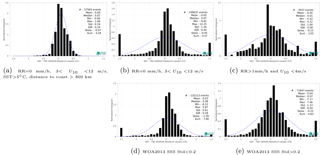
Figure 15: Normalized histogram of \Delta SSS (SMAP SSS L3 v5.0 - Monthly (JPL) - TSG (GOSUD-Research-vessel)) for 5 different subdatasets corresponding to: RR=0 mm/h, 3 < U_{10} < 12 m/s, SST>5°C, distance to coast > 800 km (a), RR=0 mm/h, 3 < U_{10} < 12 m/s (b), RR>1mm/h and U_{10} < 4 m/s (c), WOA2013 SSS Std<0.2 (d), WOA2013 SSS Std>0.2 (e).
