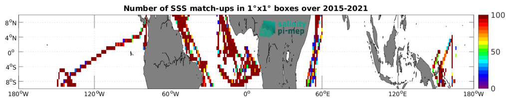
Figure 5: Number of SSS match-ups between TSG (GOSUD-Research-vessel) SSS and the SMAP SSS L3 v5.0 - Monthly (JPL) SSS product for the Equatorial Ocean 10N-10S Pi-MEP region over 1°×1° boxes and for the full satellite product period.
