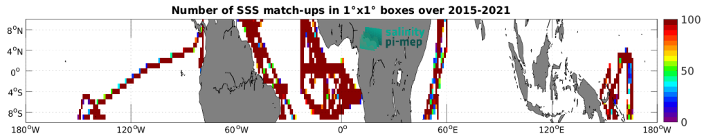
Figure 4: Number of SSS match-ups between TSG (GOSUD-Research-vessel) SSS and the SMAP SSS L3 v5.0 - Monthly (JPL) SSS product for the Equatorial Ocean 10N-10S Pi-MEP region over 1°×1° boxes and for the full satellite product period.
