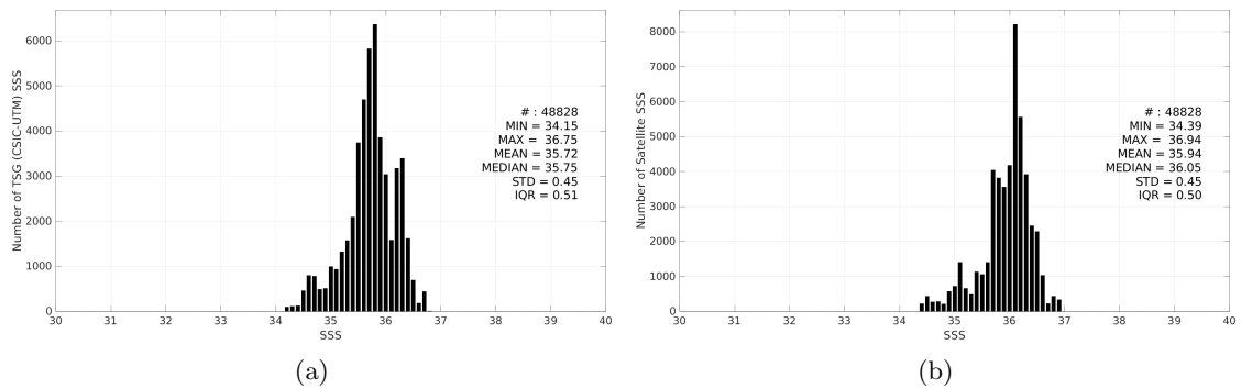
Figure 3: Histograms of SSS from TSG (CSIC-UTM) (a) and SMAP SSS L3 v5.0 - Monthly (JPL) (b) considering all match-up pairs per bins of 0.1 over the Equatorial Ocean 10N-10S Pi-MEP region and for the full satellite product period.
