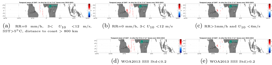
Figure 14: Temporal mean gridded over spatial boxes of size 1^\circ \times 1^\circ of \Delta SSS (SMAP SSS L3 v5.0 - Monthly (JPL) - TSG (CSIC-UTM)) for 5 different subdatasets corresponding to: RR=0 mm/h, 3 < U_{10} < 12 m/s, SST>5°C, distance to coast > 800 km (a), RR=0 mm/h, 3 < U_{10} < 12 m/s (b), RR>1mm/h and U_{10} < 4 m/s (c), WOA2013 SSS Std<0.2 (d), WOA2013 SSS Std>0.2 (e).
