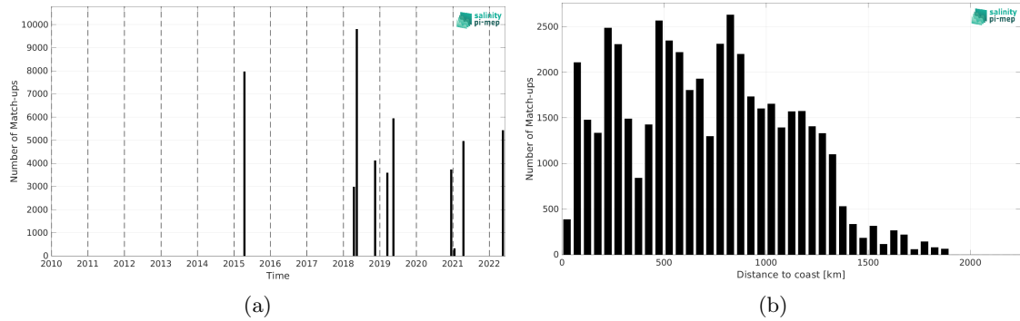
Figure 2: Number of match-ups between TSG (CSIC-UTM) and SMAP SSS L3 v5.0 - Monthly (JPL) SSS as a function of time (a) and as function of the distance to coast (b) over the Equatorial Ocean 10N-10S Pi-MEP region and for the full satellite product period.
