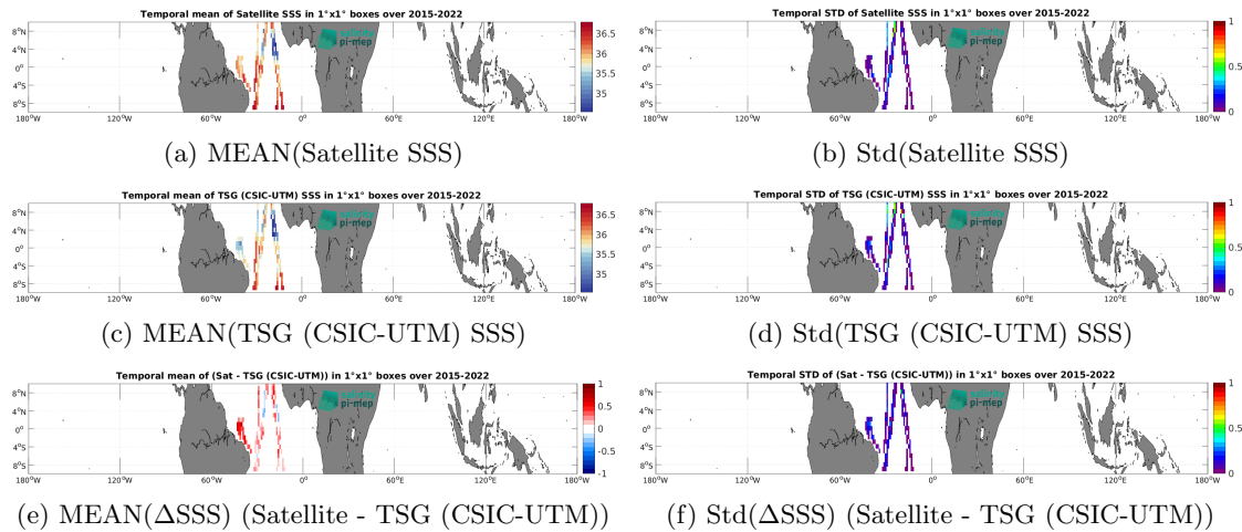
Figure 7: Temporal mean (left) and Std (right) of SSS from SMAP SSS L3 v5.0 - Monthly (JPL) (top), TSG (CSIC-UTM) (middle), and of \Delta SSS (Satellite - TSG (CSIC-UTM)). Only match-up pairs are used to generate these maps.
