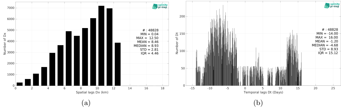
Figure 6: Histograms of the spatial (a) and temporal (b) lags between the location/time of the TSG (CSIC-UTM) measurement and the date of the corresponding SMAP SSS L3 v5.0 - Monthly (JPL) SSS pixel.
