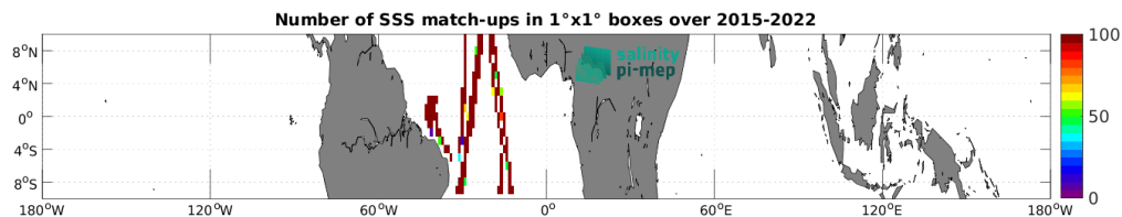
Figure 5: Number of SSS match-ups between TSG (CSIC-UTM) SSS and the SMAP SSS L3 v5.0 - Monthly (JPL) SSS product for the Equatorial Ocean 10N-10S Pi-MEP region over 1^\circ \times 1^\circ boxes and for the full satellite product period.
